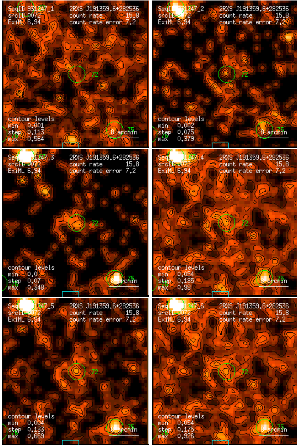
Figure 72: RASS 931247: detection 0072: band rate images, Gaussian filter: (1) PSPC channels 11 – 41, (2) 52 – 90, (3) 91 – 201, (4) 11 – 235, (5) 52 – 201, (6) 11 – 201. Broad band rates in counts/ks. Band rate contour levels in counts/ks/arcmin 2 .
