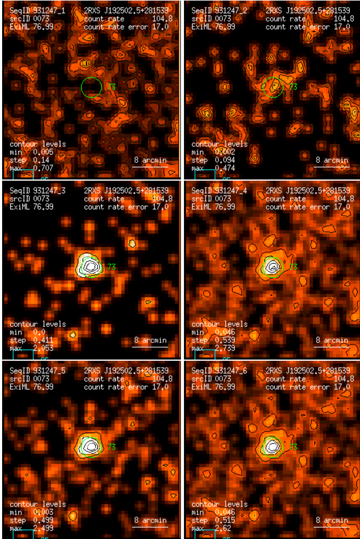
Figure 73: RASS 931247: detection 0073: band rate images, Gaussian filter: (1) PSPC channels 11 – 41, (2) 52 – 90, (3) 91 – 201, (4) 11 – 235, (5) 52 – 201, (6) 11 – 201. Broad band rates in counts/ks. Band rate contour levels in counts/ks/arcmin 2 .
