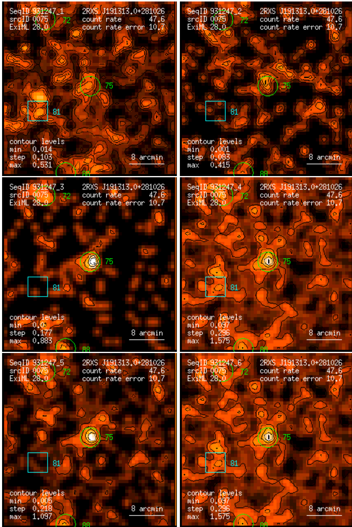
Figure 75: RASS 931247: detection 0075: band rate images, Gaussian filter: (1) PSPC channels 11 – 41, (2) 52 – 90, (3) 91 – 201, (4) 11 – 235, (5) 52 – 201, (6) 11 – 201. Broad band rates in counts/ks. Band rate contour levels in counts/ks/arcmin 2 .
