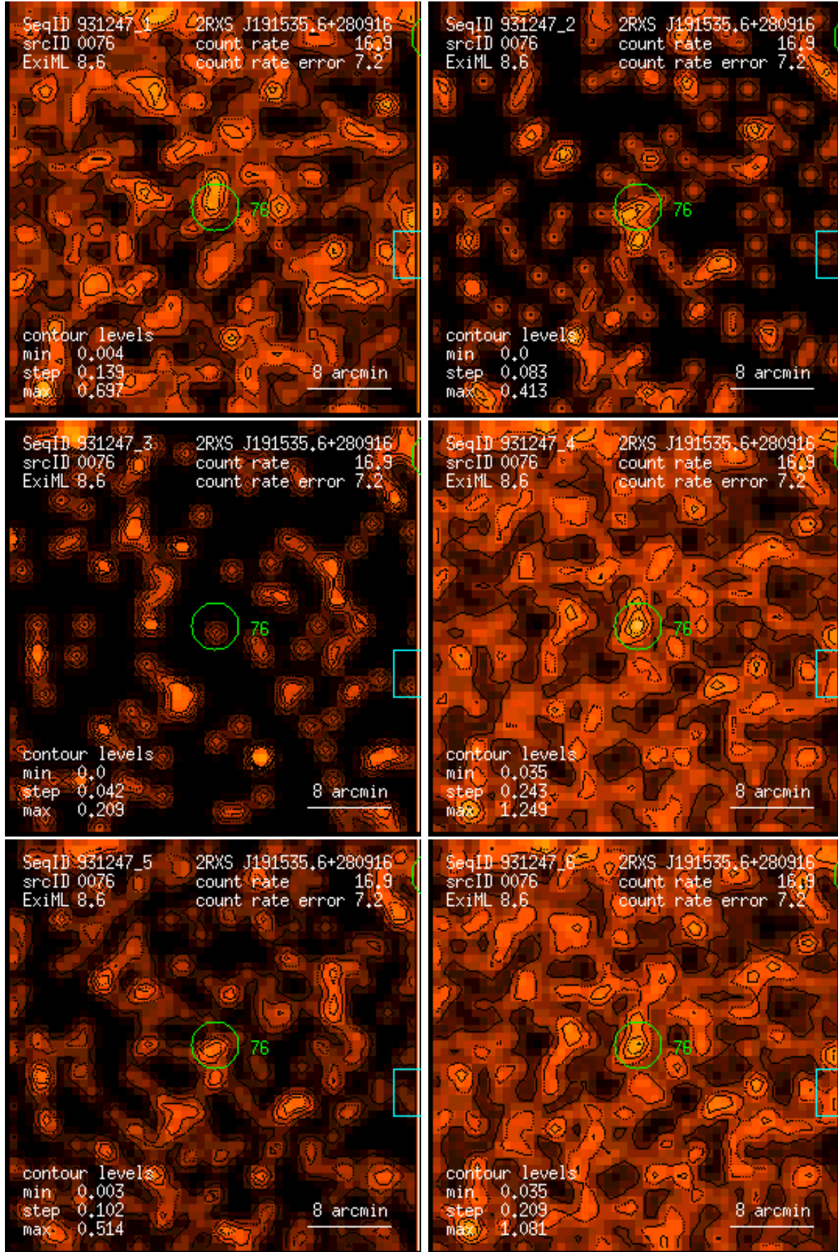
Figure 76: RASS 931247: detection 0076: band rate images, Gaussian filter: (1) PSPC channels 11 – 41, (2) 52 – 90, (3) 91 – 201, (4) 11 – 235, (5) 52 – 201, (6) 11 – 201. Broad band rates in counts/ks. Band rate contour levels in counts/ks/arcmin 2 .
