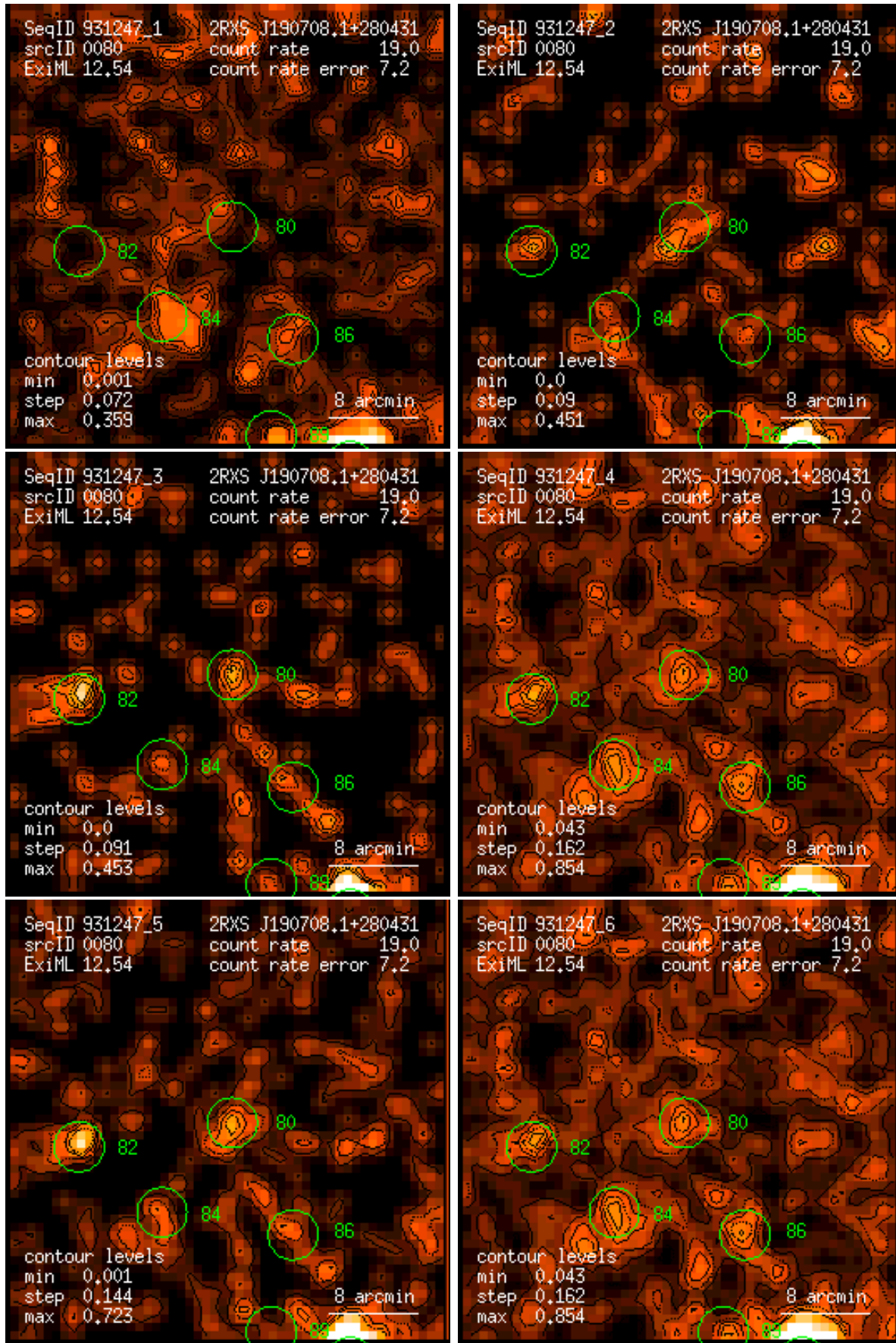
Figure 80: RASS 931247: detection 0080: band rate images, Gaussian filter: (1) PSPC channels 11 – 41, (2) 52 – 90, (3) 91 – 201, (4) 11 – 235, (5) 52 – 201, (6) 11 – 201. Broad band rates in counts/ks. Band rate contour levels in counts/ks/arcmin 2 .
