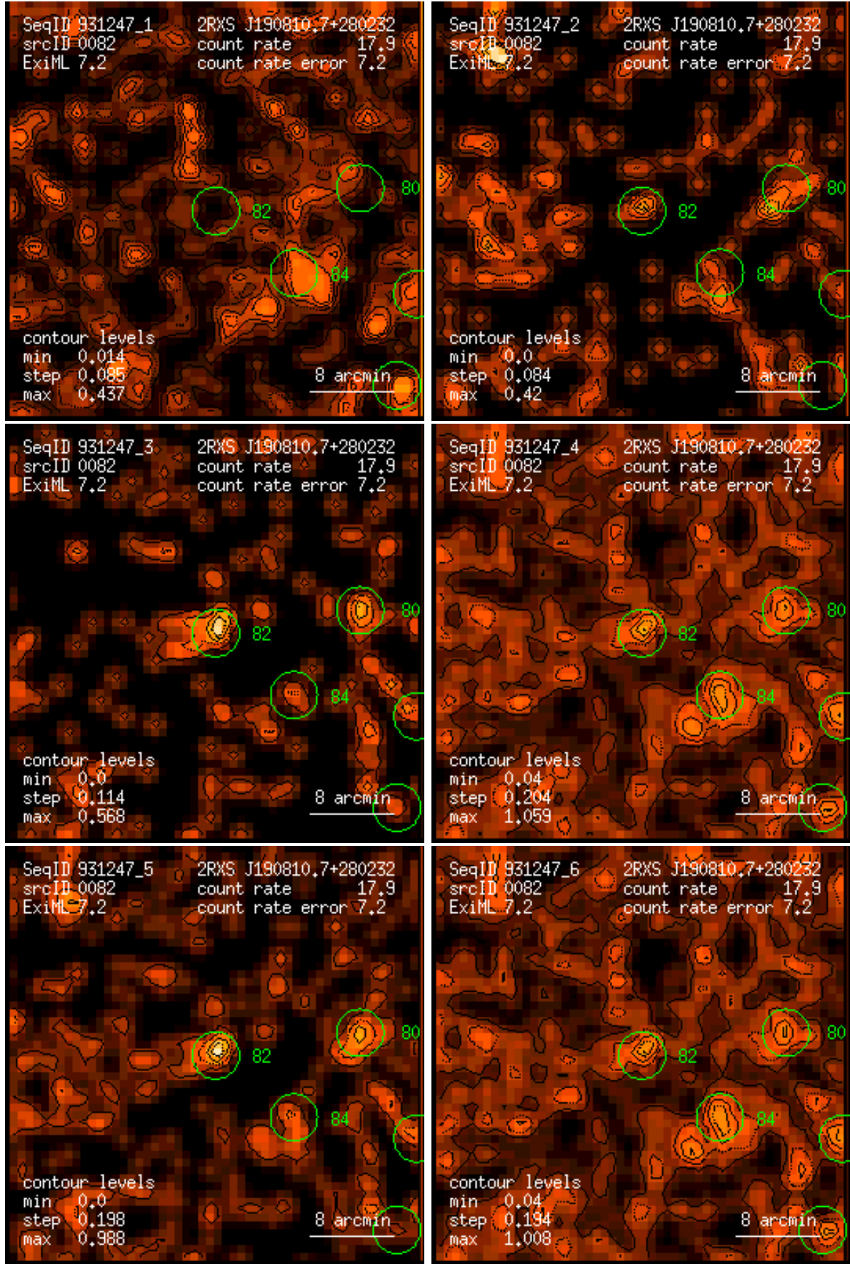
Figure 82: RASS 931247: detection 0082: band rate images, Gaussian filter: (1) PSPC channels 11 – 41, (2) 52 – 90, (3) 91 – 201, (4) 11 – 235, (5) 52 – 201, (6) 11 – 201. Broad band rates in counts/ks. Band rate contour levels in counts/ks/arcmin 2 .
