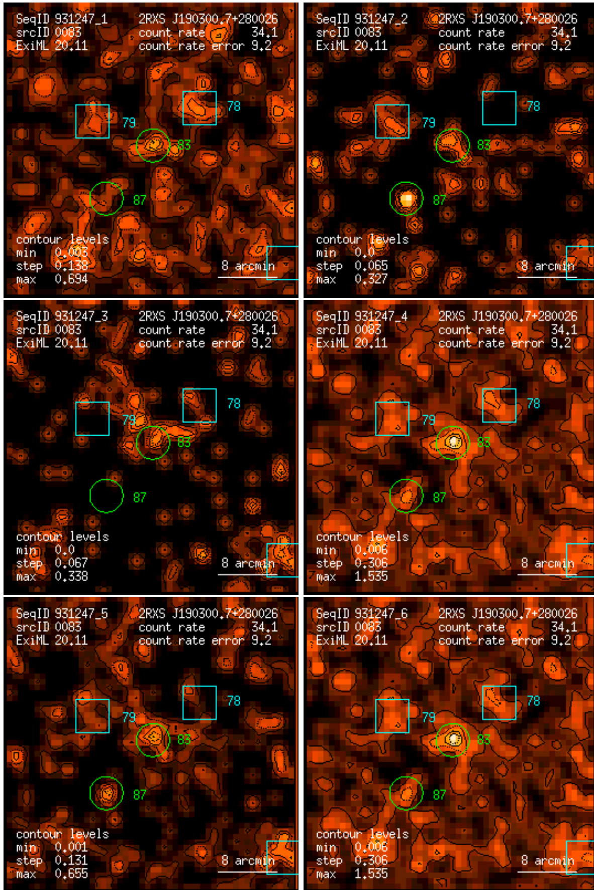
Figure 83: RASS 931247: detection 0083: band rate images, Gaussian filter: (1) PSPC channels 11 – 41, (2) 52 – 90, (3) 91 – 201, (4) 11 – 235, (5) 52 – 201, (6) 11 – 201. Broad band rates in counts/ks. Band rate contour levels in counts/ks/arcmin 2 .
