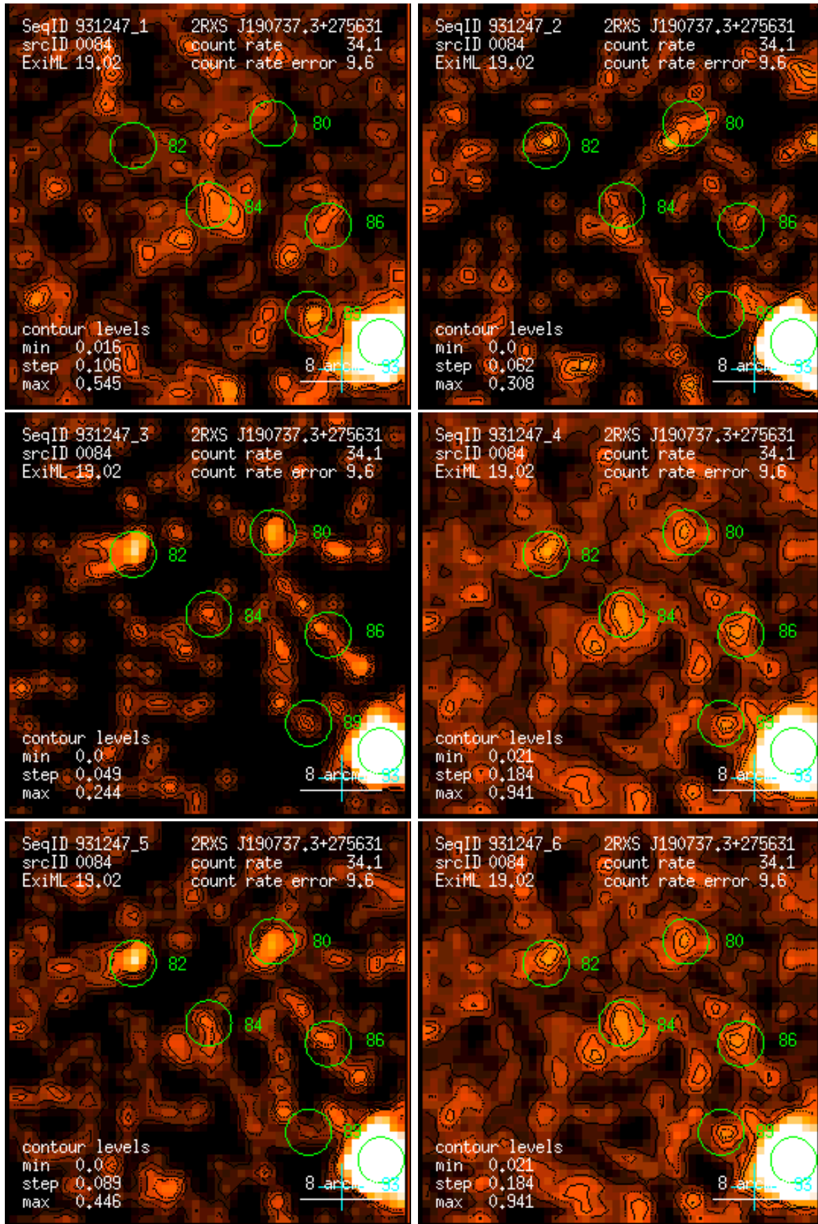
Figure 84: RASS 931247: detection 0084: band rate images, Gaussian filter: (1) PSPC channels 11 – 41, (2) 52 – 90, (3) 91 – 201, (4) 11 – 235, (5) 52 – 201, (6) 11 – 201. Broad band rates in counts/ks. Band rate contour levels in counts/ks/arcmin 2 .
