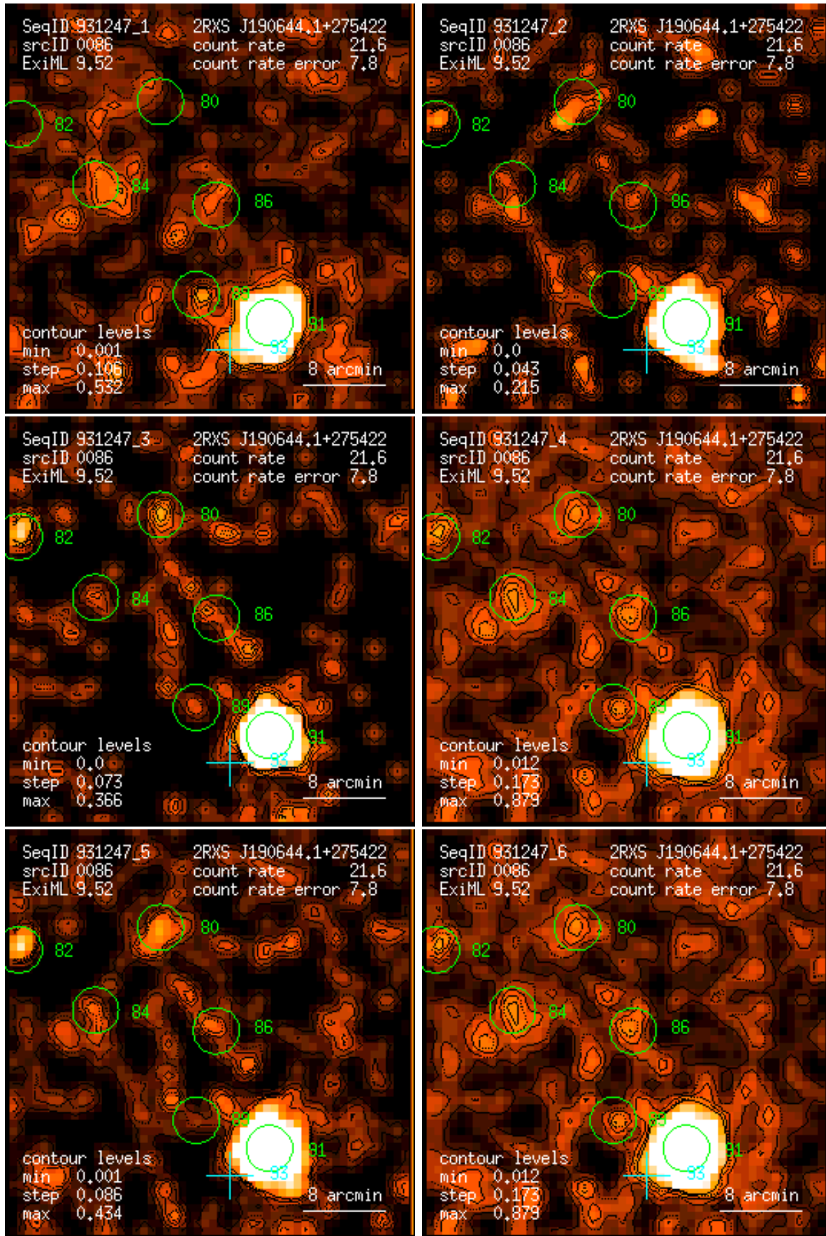
Figure 86: RASS 931247: detection 0086: band rate images, Gaussian filter: (1) PSPC channels 11 – 41, (2) 52 – 90, (3) 91 – 201, (4) 11 – 235, (5) 52 – 201, (6) 11 – 201. Broad band rates in counts/ks. Band rate contour levels in counts/ks/arcmin 2 .
