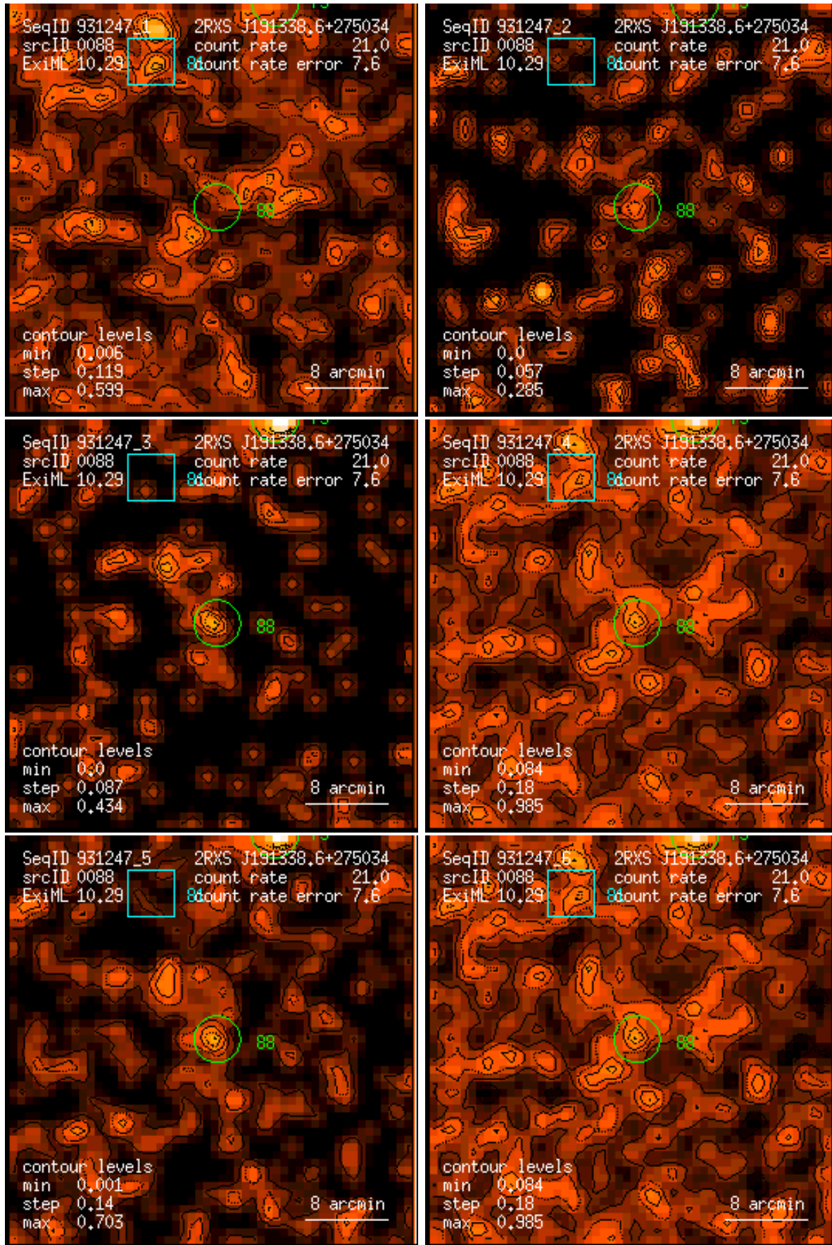
Figure 88: RASS 931247: detection 0088: band rate images, Gaussian filter: (1) PSPC channels 11 – 41, (2) 52 – 90, (3) 91 – 201, (4) 11 – 235, (5) 52 – 201, (6) 11 – 201. Broad band rates in counts/ks. Band rate contour levels in counts/ks/arcmin 2 .
