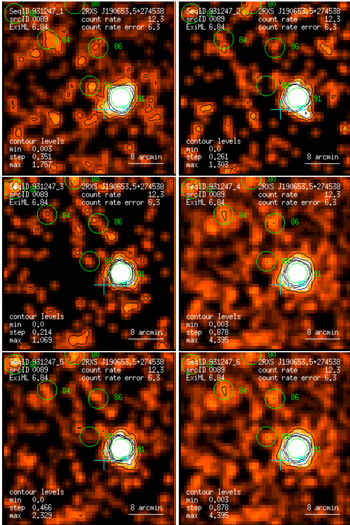
Figure 89: RASS 931247: detection 0089: band rate images, Gaussian filter: (1) PSPC channels 11 – 41, (2) 52 – 90, (3) 91 – 201, (4) 11 – 235, (5) 52 – 201, (6) 11 – 201. Broad band rates in counts/ks. Band rate contour levels in counts/ks/arcmin 2 .
