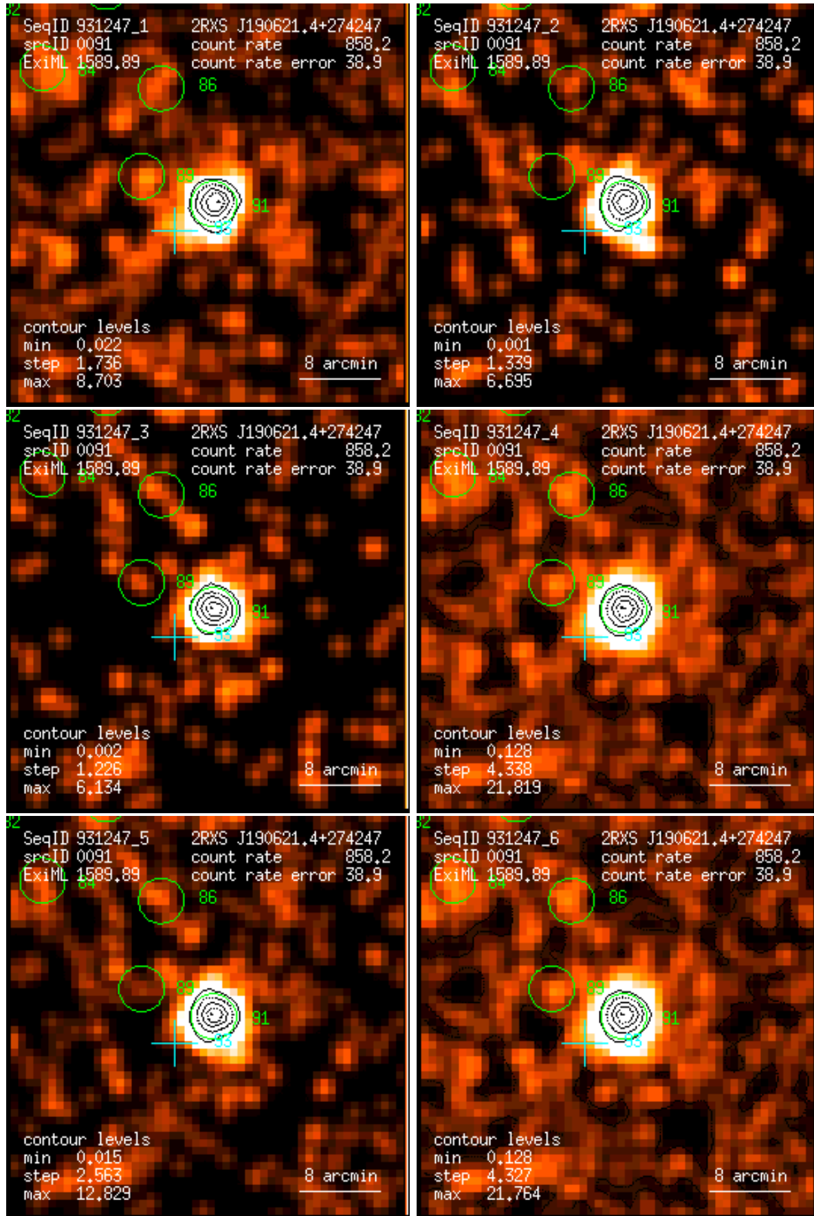
Figure 91: RASS 931247: detection 0091: band rate images, Gaussian filter: (1) PSPC channels 11 – 41, (2) 52 – 90, (3) 91 – 201, (4) 11 – 235, (5) 52 – 201, (6) 11 – 201. Broad band rates in counts/ks. Band rate contour levels in counts/ks/arcmin 2 .
