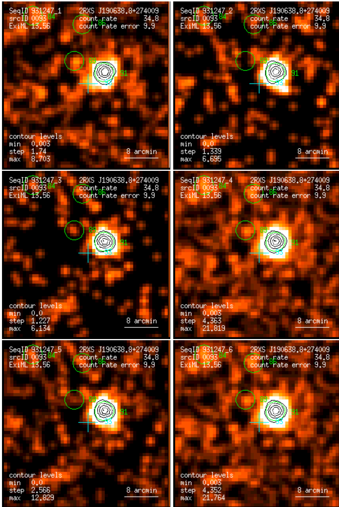
Figure 93: RASS 931247: detection 0093: band rate images, Gaussian filter: (1) PSPC channels 11 – 41, (2) 52 – 90, (3) 91 – 201, (4) 11 – 235, (5) 52 – 201, (6) 11 – 201. Broad band rates in counts/ks. Band rate contour levels in counts/ks/arcmin 2 .
