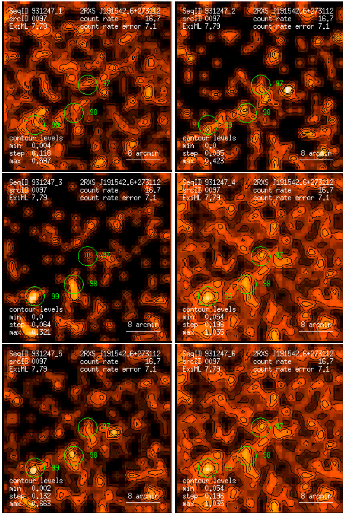
Figure 97: RASS 931247: detection 0097: band rate images, Gaussian filter: (1) PSPC channels 11 – 41, (2) 52 – 90, (3) 91 – 201, (4) 11 – 235, (5) 52 – 201, (6) 11 – 201. Broad band rates in counts/ks. Band rate contour levels in counts/ks/arcmin 2 .
