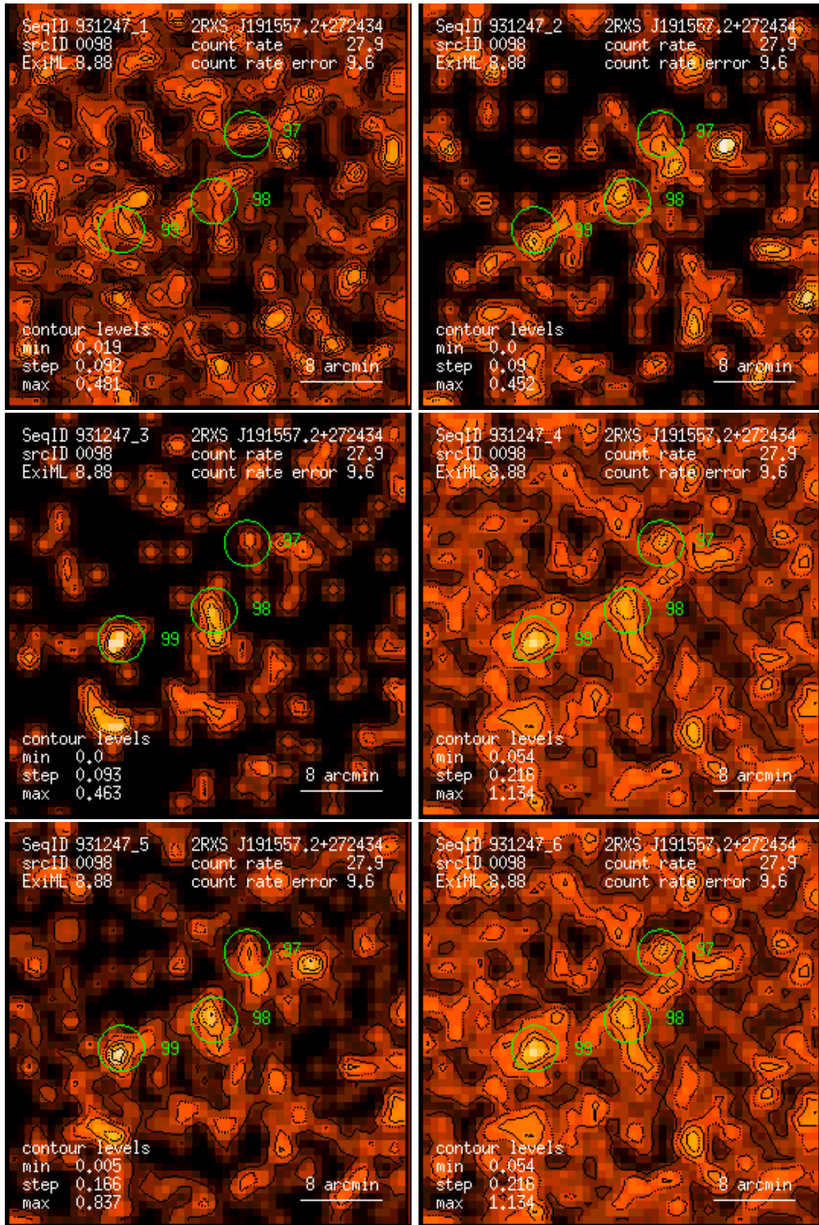
Figure 98: RASS 931247: detection 0098: band rate images, Gaussian filter: (1) PSPC channels 11 – 41, (2) 52 – 90, (3) 91 – 201, (4) 11 – 235, (5) 52 – 201, (6) 11 – 201. Broad band rates in counts/ks. Band rate contour levels in counts/ks/arcmin 2 .
