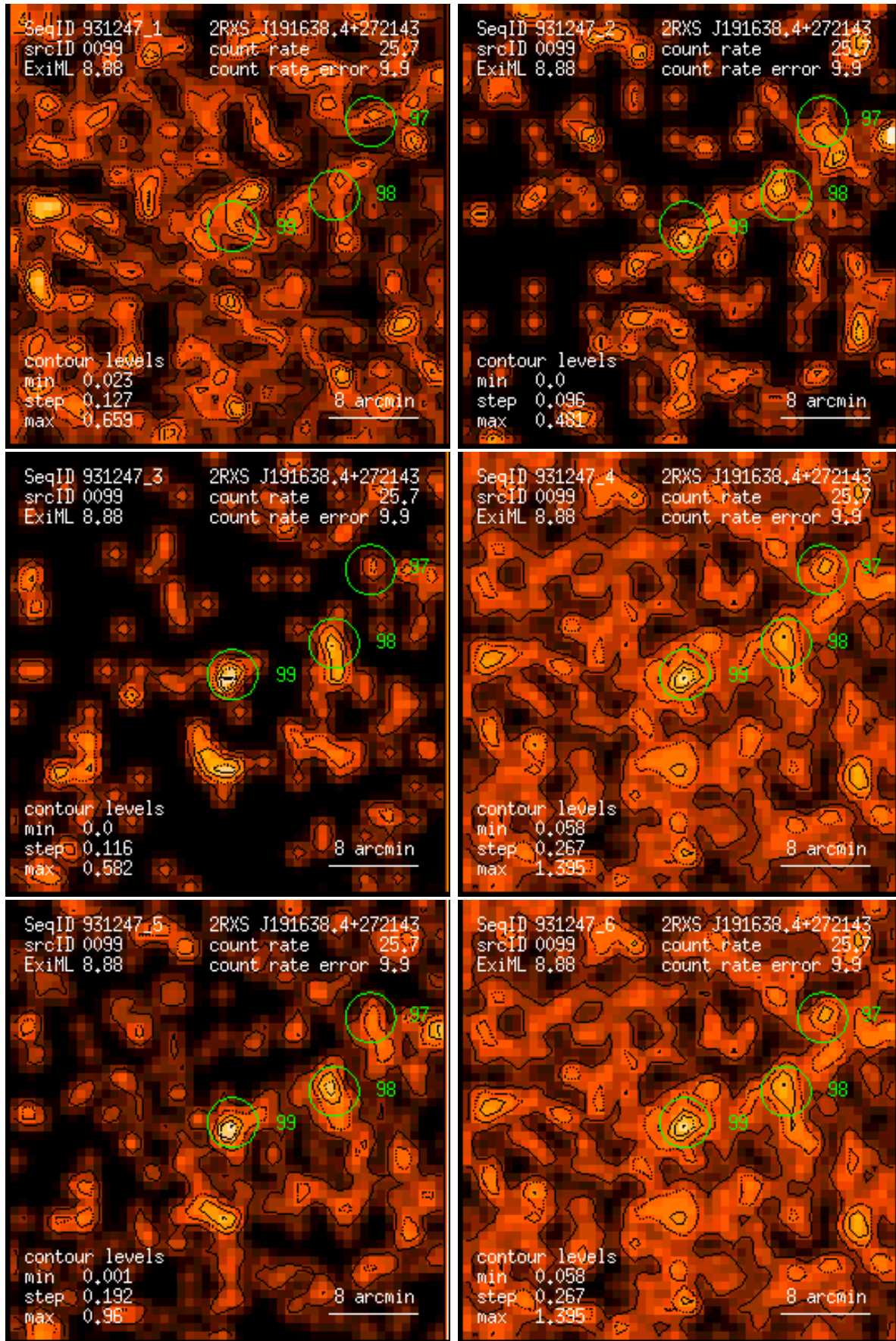
Figure 99: RASS 931247: detection 0099: band rate images, Gaussian filter: (1) PSPC channels 11 – 41, (2) 52 – 90, (3) 91 – 201, (4) 11 – 235, (5) 52 – 201, (6) 11 – 201. Broad band rates in counts/ks. Band rate contour levels in counts/ks/arcmin 2 .
