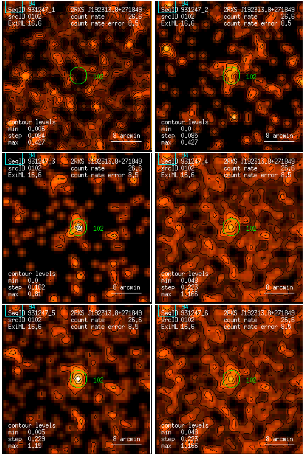
Figure 102: RASS 931247: detection 0102: band rate images, Gaussian filter: (1) PSPC channels 11 – 41, (2) 52 – 90, (3) 91 – 201, (4) 11 – 235, (5) 52 – 201, (6) 11 – 201. Broad band rates in counts/ks. Band rate contour levels in counts/ks/arcmin 2 .
