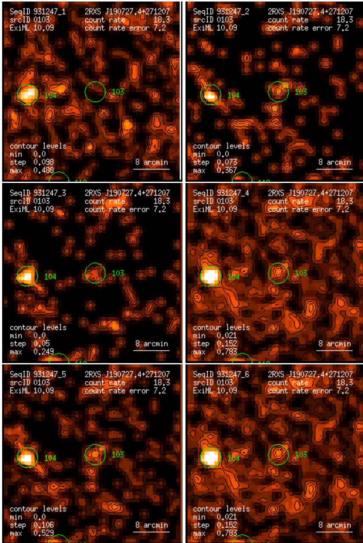
Figure 103: RASS 931247: detection 0103: band rate images, Gaussian filter: (1) PSPC channels 11 – 41, (2) 52 – 90, (3) 91 – 201, (4) 11 – 235, (5) 52 – 201, (6) 11 – 201. Broad band rates in counts/ks. Band rate contour levels in counts/ks/arcmin 2 .
