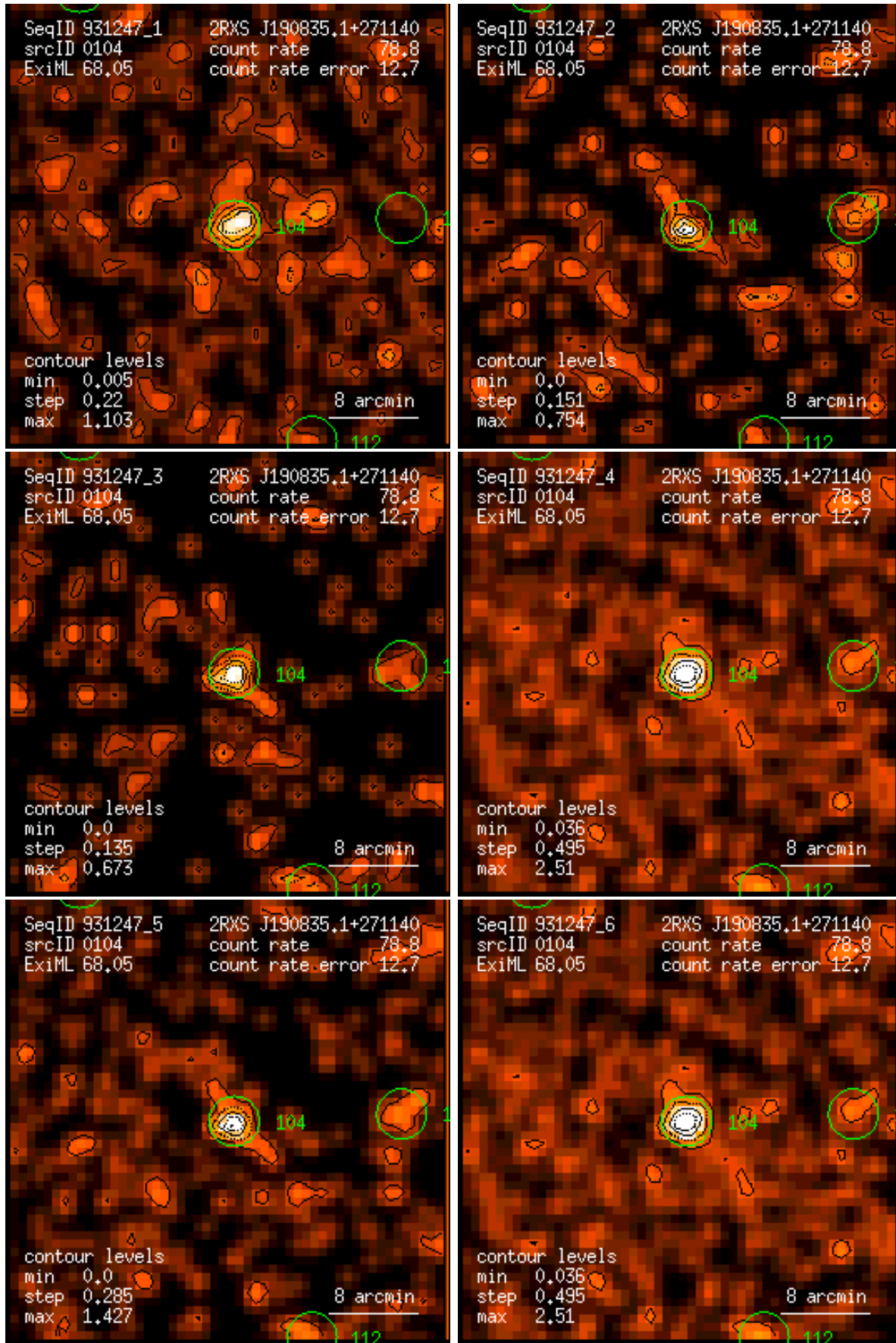
Figure 104: RASS 931247: detection 0104: band rate images, Gaussian filter: (1) PSPC channels 11 – 41, (2) 52 – 90, (3) 91 – 201, (4) 11 – 235, (5) 52 – 201, (6) 11 – 201. Broad band rates in counts/ks. Band rate contour levels in counts/ks/arcmin 2 .
