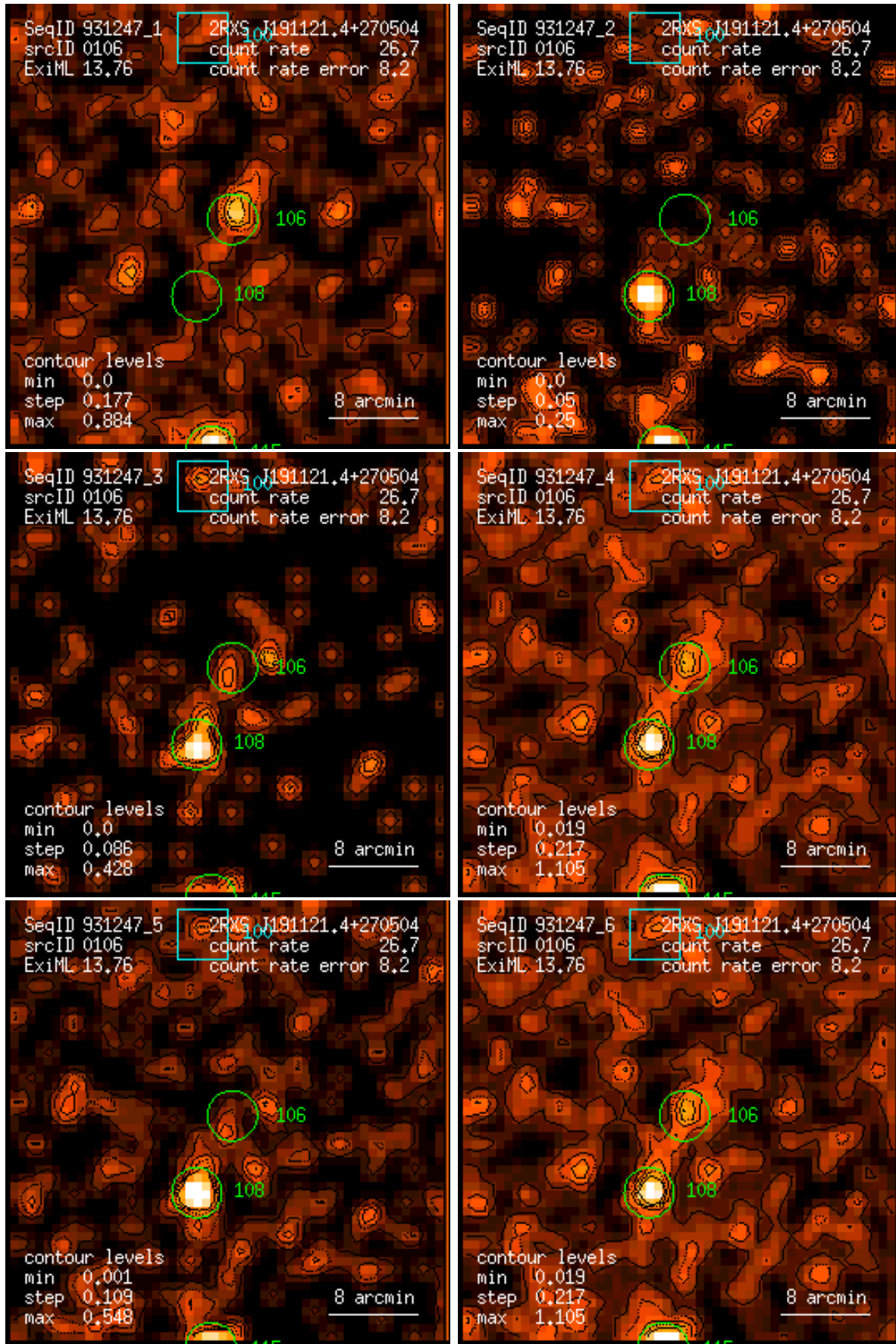
Figure 106: RASS 931247: detection 0106: band rate images, Gaussian filter: (1) PSPC channels 11 – 41, (2) 52 – 90, (3) 91 – 201, (4) 11 – 235, (5) 52 – 201, (6) 11 – 201. Broad band rates in counts/ks. Band rate contour levels in counts/ks/arcmin 2 .
