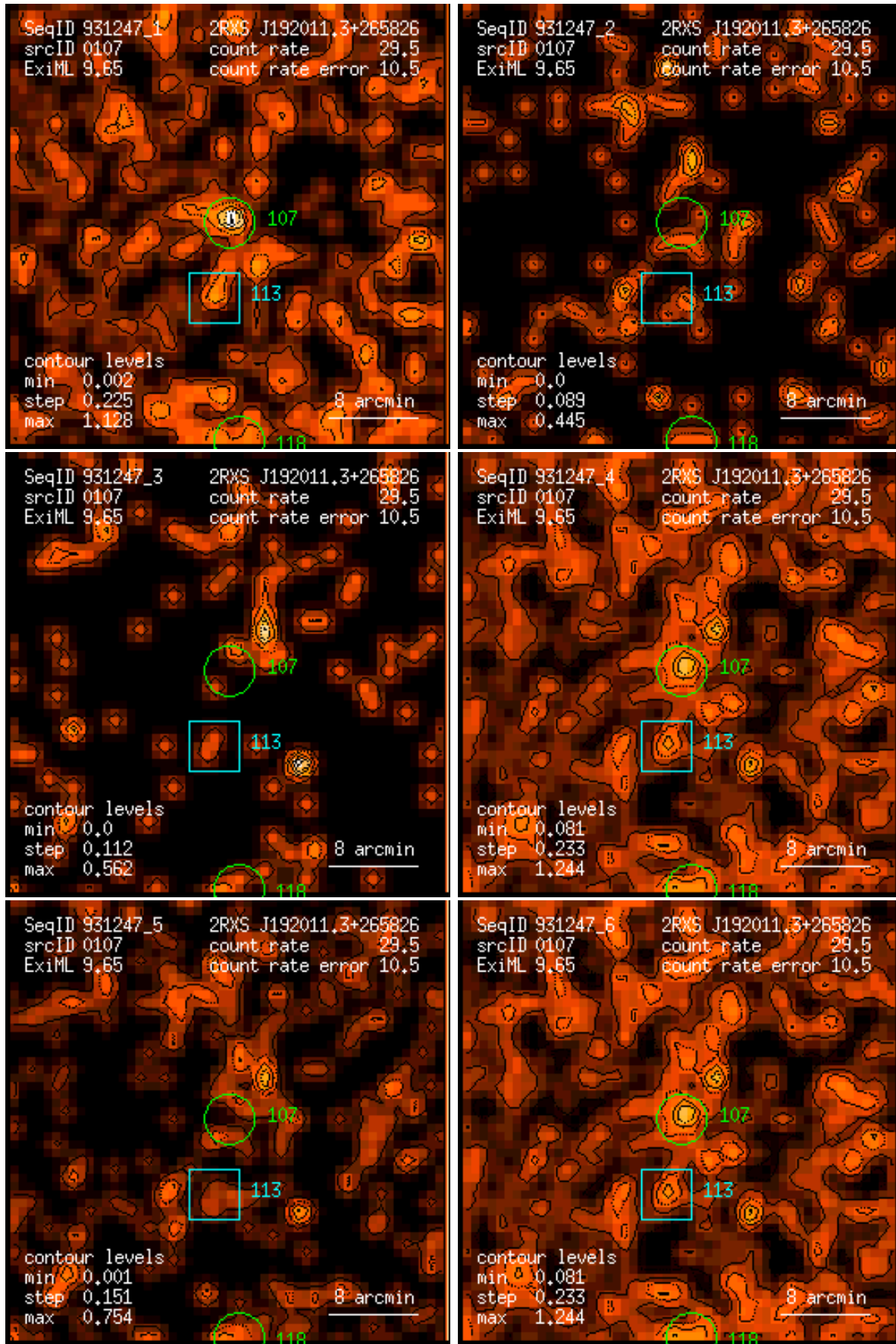
Figure 107: RASS 931247: detection 0107: band rate images, Gaussian filter: (1) PSPC channels 11 – 41, (2) 52 – 90, (3) 91 – 201, (4) 11 – 235, (5) 52 – 201, (6) 11 – 201. Broad band rates in counts/ks. Band rate contour levels in counts/ks/arcmin 2 .
