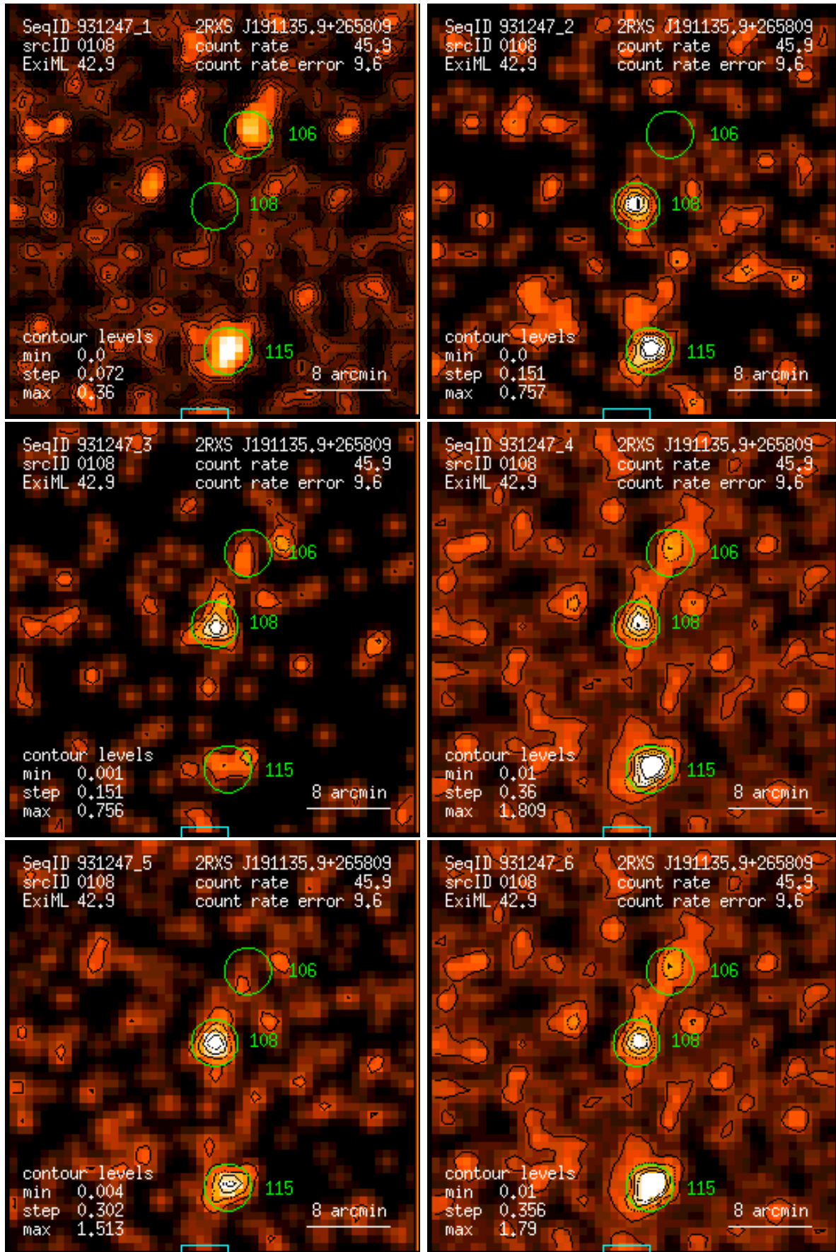
Figure 108: RASS 931247: detection 0108: band rate images, Gaussian filter: (1) PSPC channels 11 – 41, (2) 52 – 90, (3) 91 – 201, (4) 11 – 235, (5) 52 – 201, (6) 11 – 201. Broad band rates in counts/ks. Band rate contour levels in counts/ks/arcmin 2 .
