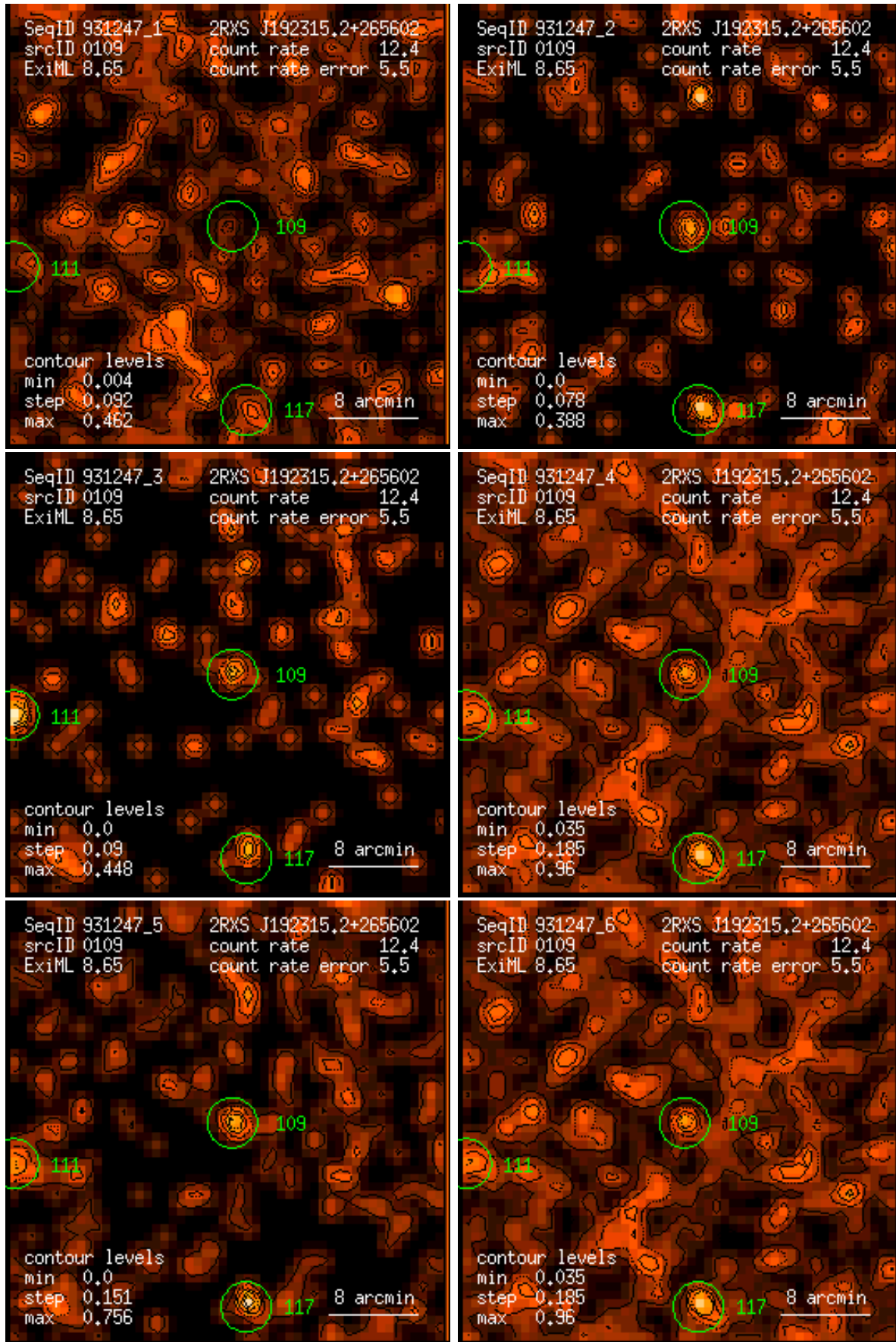
Figure 109: RASS 931247: detection 0109: band rate images, Gaussian filter: (1) PSPC channels 11 – 41, (2) 52 – 90, (3) 91 – 201, (4) 11 – 235, (5) 52 – 201, (6) 11 – 201. Broad band rates in counts/ks. Band rate contour levels in counts/ks/arcmin 2 .
