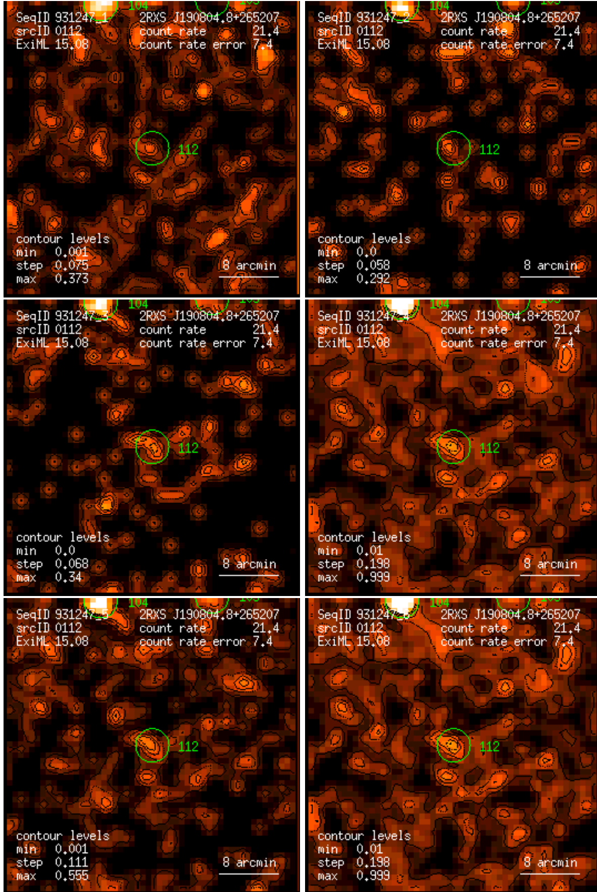
Figure 112: RASS 931247: detection 0112: band rate images, Gaussian filter: (1) PSPC channels 11 – 41, (2) 52 – 90, (3) 91 – 201, (4) 11 – 235, (5) 52 – 201, (6) 11 – 201. Broad band rates in counts/ks. Band rate contour levels in counts/ks/arcmin 2 .
