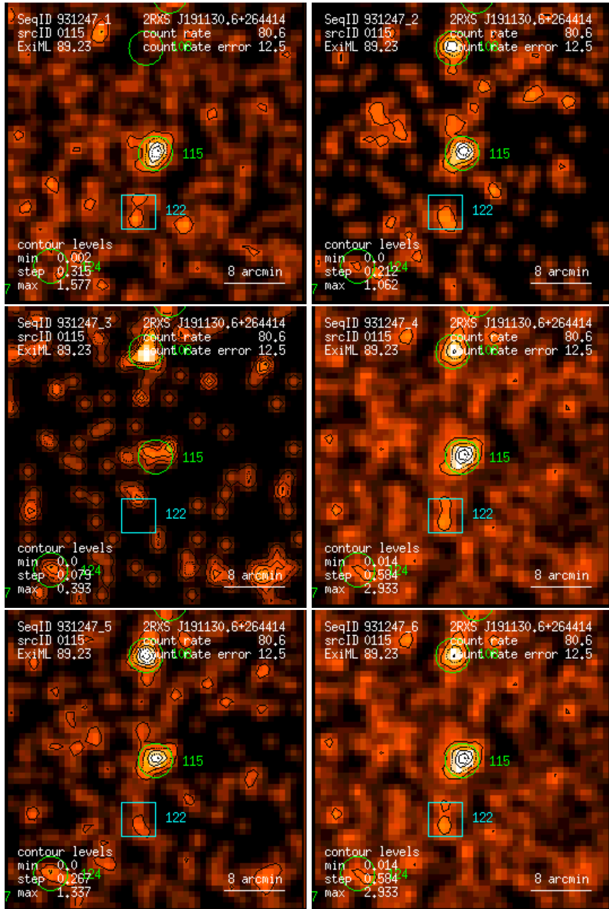
Figure 115: RASS 931247: detection 0115: band rate images, Gaussian filter: (1) PSPC channels 11 – 41, (2) 52 – 90, (3) 91 – 201, (4) 11 – 235, (5) 52 – 201, (6) 11 – 201. Broad band rates in counts/ks. Band rate contour levels in counts/ks/arcmin 2 .
