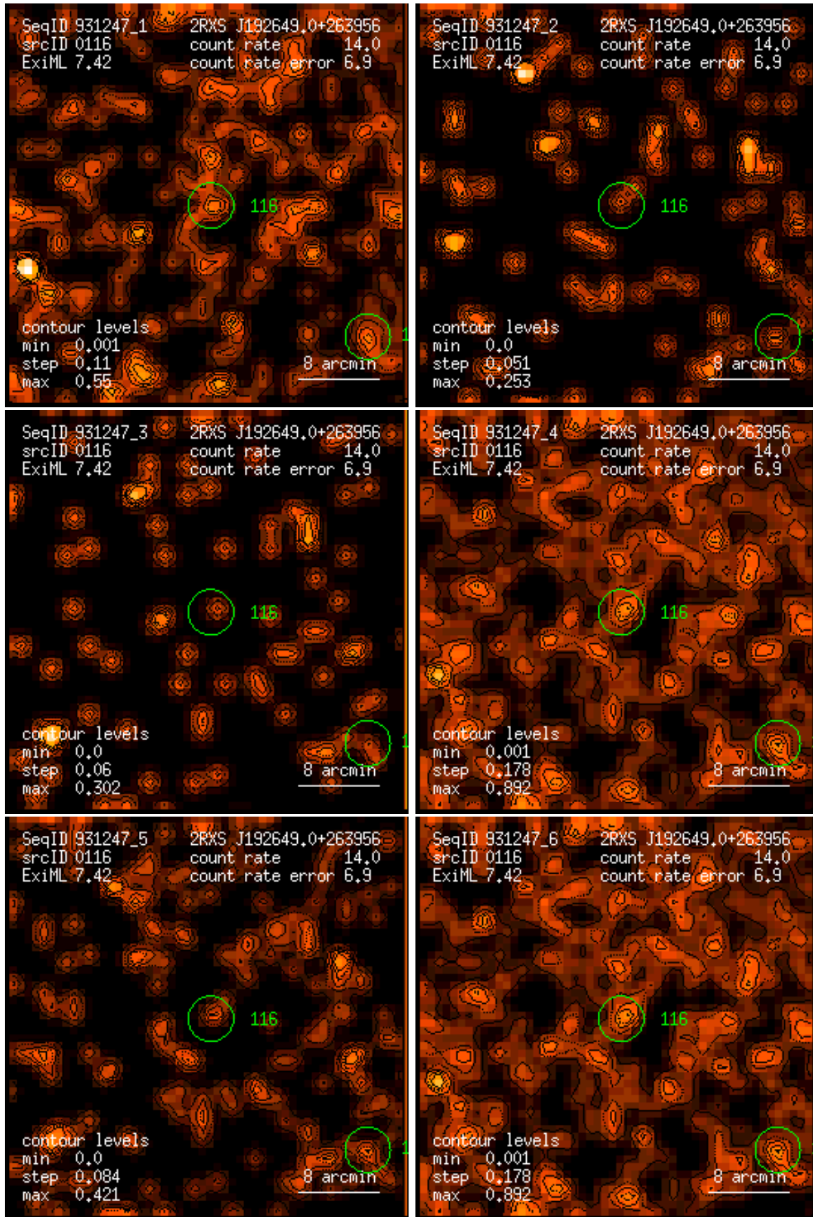
Figure 116: RASS 931247: detection 0116: band rate images, Gaussian filter: (1) PSPC channels 11 – 41, (2) 52 – 90, (3) 91 – 201, (4) 11 – 235, (5) 52 – 201, (6) 11 – 201. Broad band rates in counts/ks. Band rate contour levels in counts/ks/arcmin 2 .
