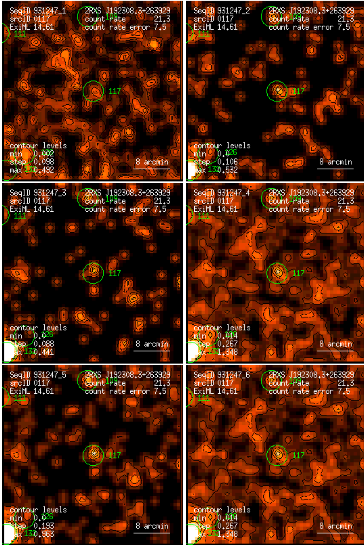
Figure 117: RASS 931247: detection 0117: band rate images, Gaussian filter: (1) PSPC channels 11 – 41, (2) 52 – 90, (3) 91 – 201, (4) 11 – 235, (5) 52 – 201, (6) 11 – 201. Broad band rates in counts/ks. Band rate contour levels in counts/ks/arcmin 2 .
