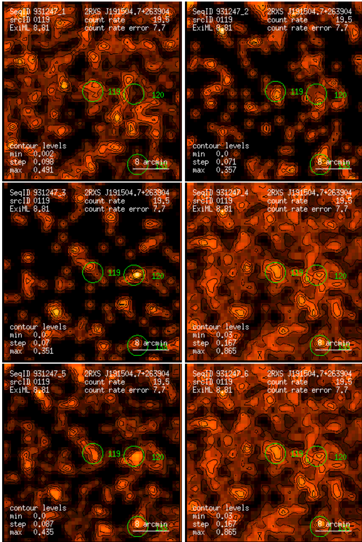
Figure 119: RASS 931247: detection 0119: band rate images, Gaussian filter: (1) PSPC channels 11 – 41, (2) 52 – 90, (3) 91 – 201, (4) 11 – 235, (5) 52 – 201, (6) 11 – 201. Broad band rates in counts/ks. Band rate contour levels in counts/ks/arcmin 2 .
