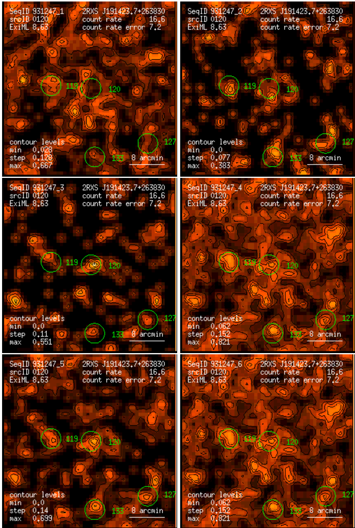
Figure 120: RASS 931247: detection 0120: band rate images, Gaussian filter: (1) PSPC channels 11 – 41, (2) 52 – 90, (3) 91 – 201, (4) 11 – 235, (5) 52 – 201, (6) 11 – 201. Broad band rates in counts/ks. Band rate contour levels in counts/ks/arcmin 2 .
