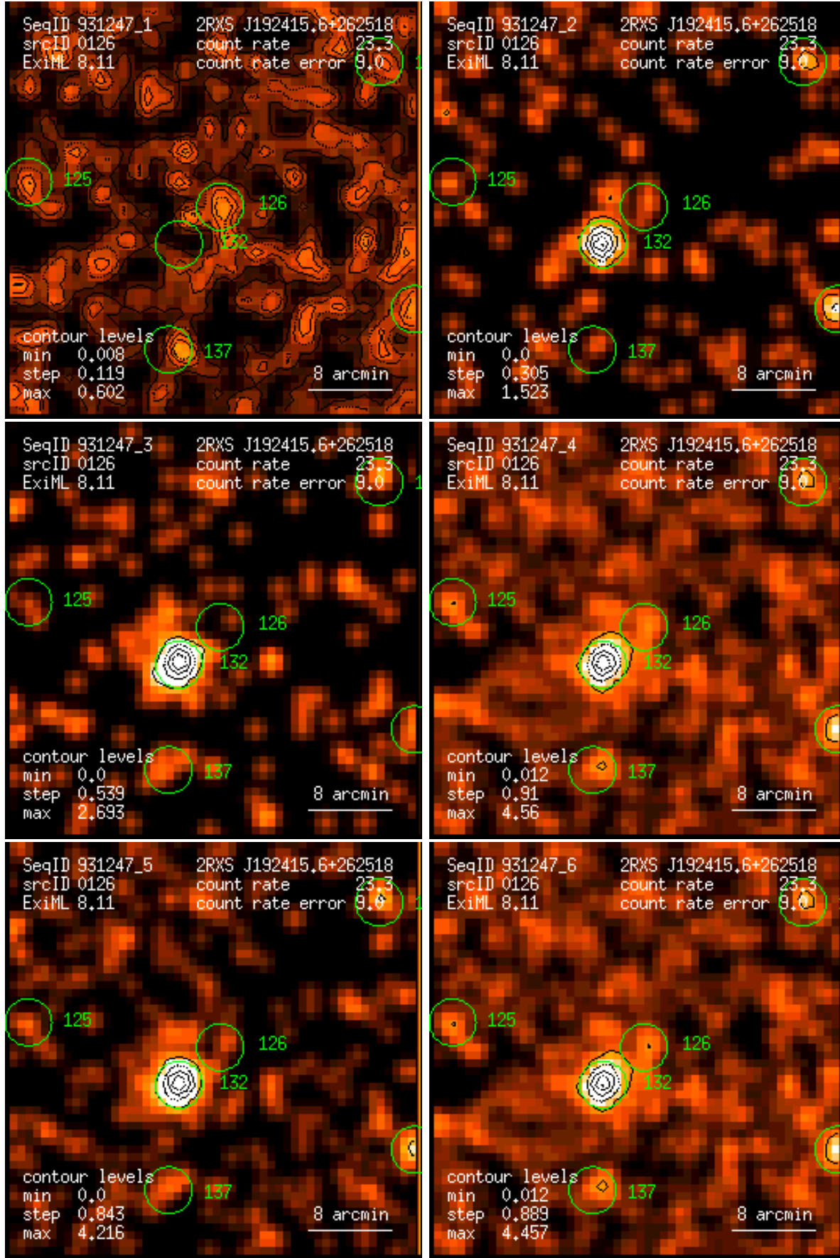
Figure 126: RASS 931247: detection 0126: band rate images, Gaussian filter: (1) PSPC channels 11 – 41, (2) 52 – 90, (3) 91 – 201, (4) 11 – 235, (5) 52 – 201, (6) 11 – 201. Broad band rates in counts/ks. Band rate contour levels in counts/ks/arcmin 2 .
