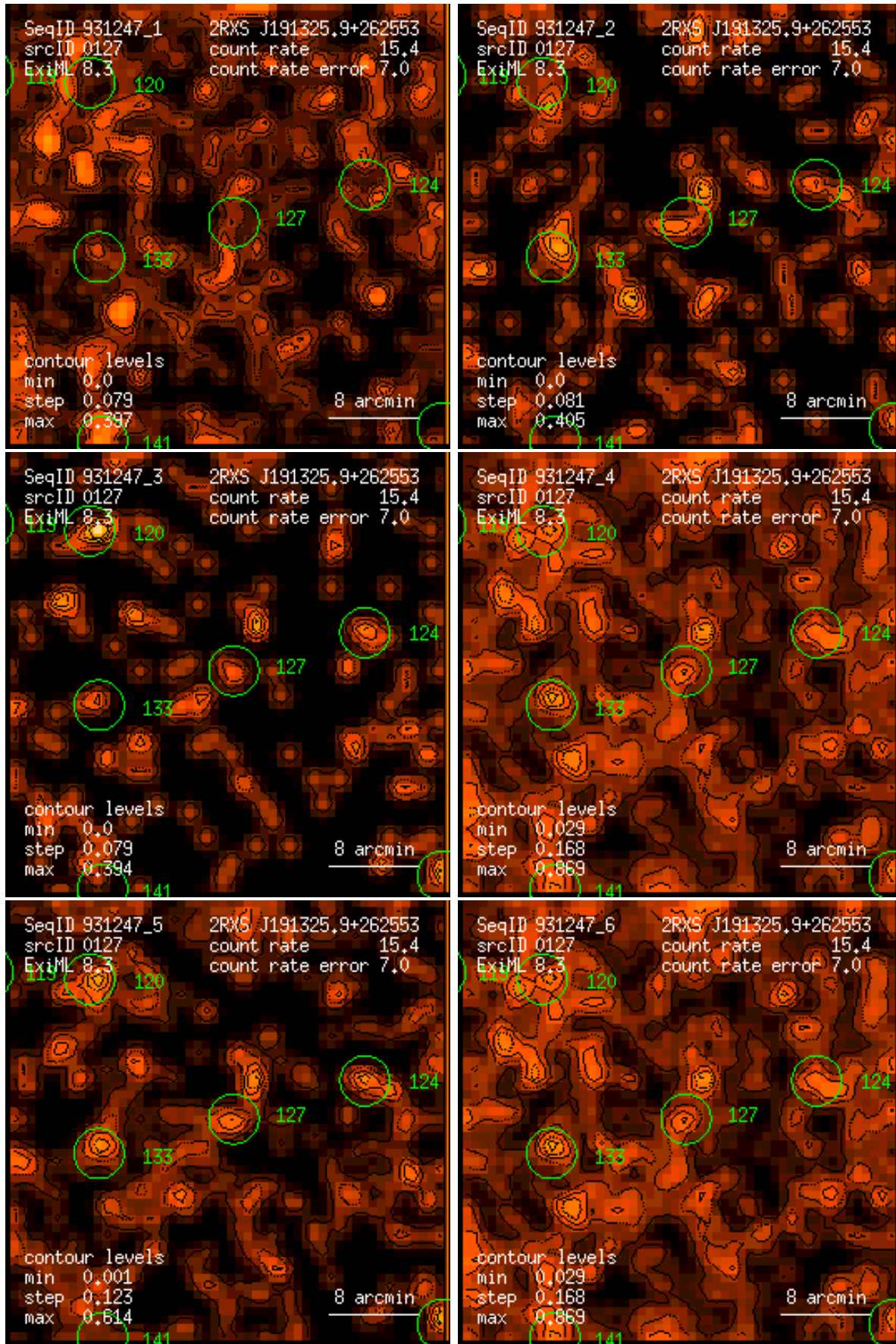
Figure 127: RASS 931247: detection 0127: band rate images, Gaussian filter: (1) PSPC channels 11 – 41, (2) 52 – 90, (3) 91 – 201, (4) 11 – 235, (5) 52 – 201, (6) 11 – 201. Broad band rates in counts/ks. Band rate contour levels in counts/ks/arcmin 2 .
