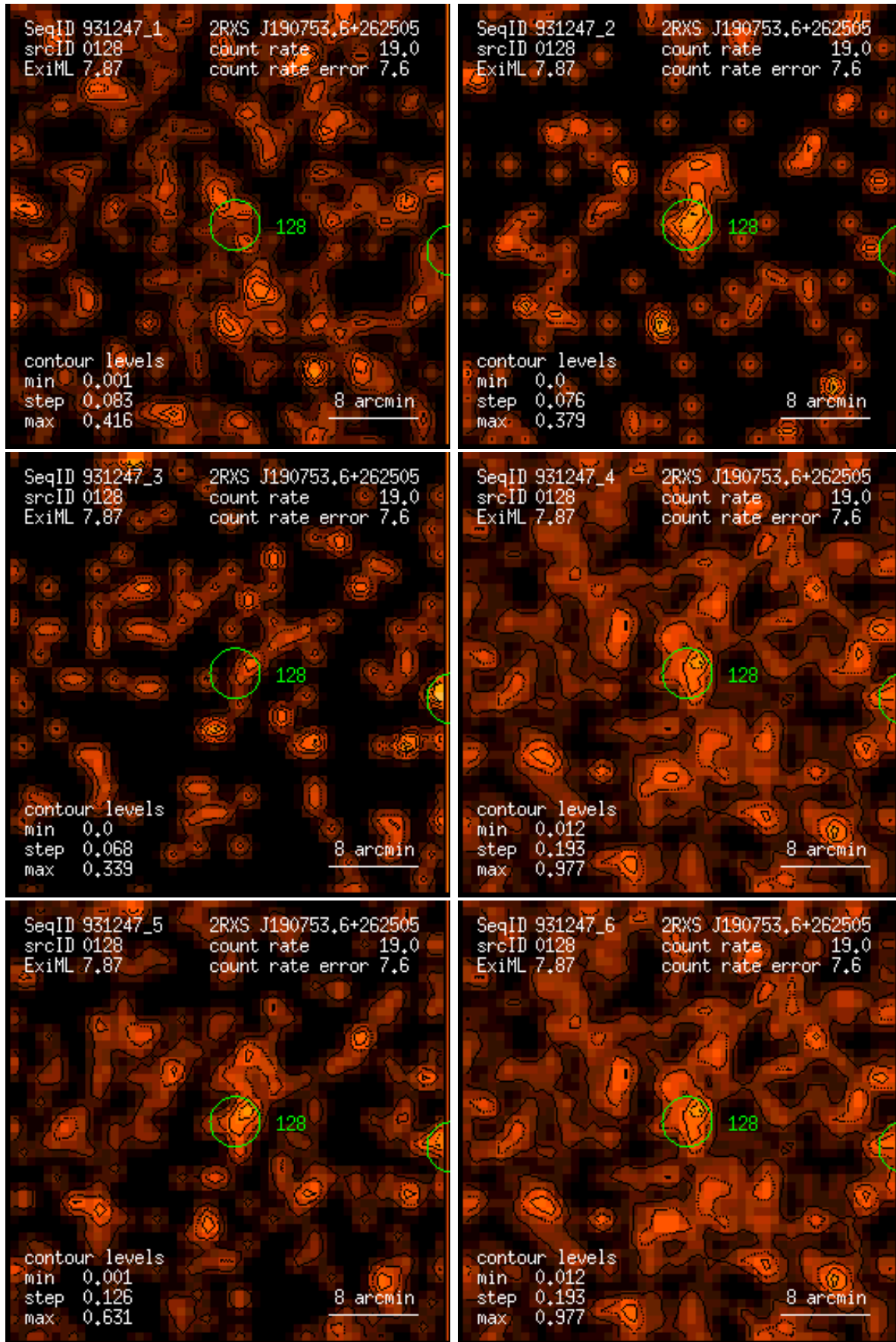
Figure 128: RASS 931247: detection 0128: band rate images, Gaussian filter: (1) PSPC channels 11 – 41, (2) 52 – 90, (3) 91 – 201, (4) 11 – 235, (5) 52 – 201, (6) 11 – 201. Broad band rates in counts/ks. Band rate contour levels in counts/ks/arcmin 2 .
