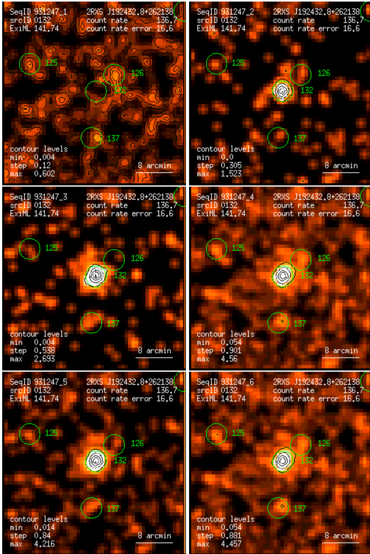
Figure 132: RASS 931247: detection 0132: band rate images, Gaussian filter: (1) PSPC channels 11 – 41, (2) 52 – 90, (3) 91 – 201, (4) 11 – 235, (5) 52 – 201, (6) 11 – 201. Broad band rates in counts/ks. Band rate contour levels in counts/ks/arcmin 2 .
