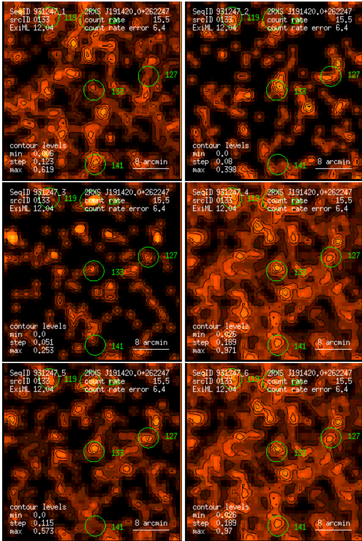
Figure 133: RASS 931247: detection 0133: band rate images, Gaussian filter: (1) PSPC channels 11 – 41, (2) 52 – 90, (3) 91 – 201, (4) 11 – 235, (5) 52 – 201, (6) 11 – 201. Broad band rates in counts/ks. Band rate contour levels in counts/ks/arcmin 2 .
