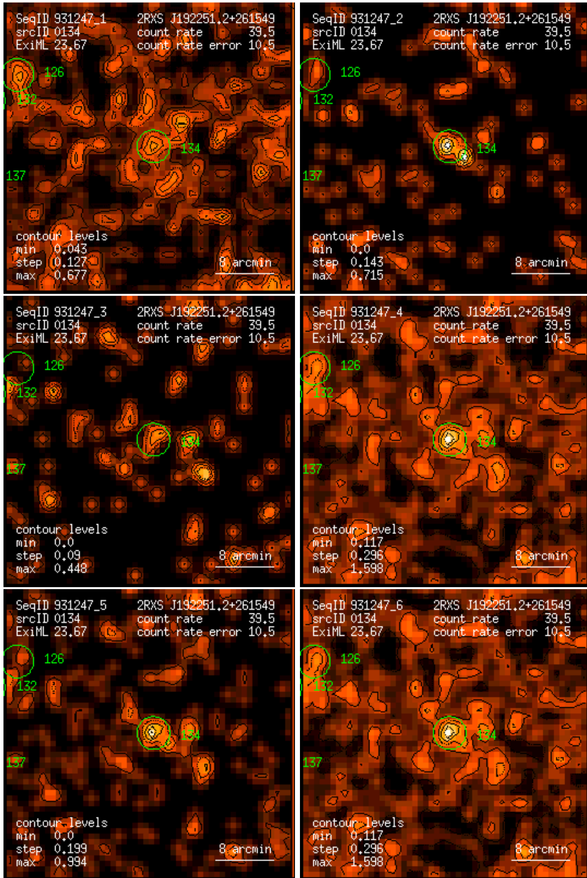
Figure 134: RASS 931247: detection 0134: band rate images, Gaussian filter: (1) PSPC channels 11 – 41, (2) 52 – 90, (3) 91 – 201, (4) 11 – 235, (5) 52 – 201, (6) 11 – 201. Broad band rates in counts/ks. Band rate contour levels in counts/ks/arcmin 2 .
