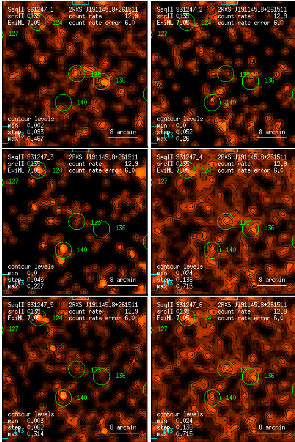
Figure 135: RASS 931247: detection 0135: band rate images, Gaussian filter: (1) PSPC channels 11 – 41, (2) 52 – 90, (3) 91 – 201, (4) 11 – 235, (5) 52 – 201, (6) 11 – 201. Broad band rates in counts/ks. Band rate contour levels in counts/ks/arcmin 2 .
