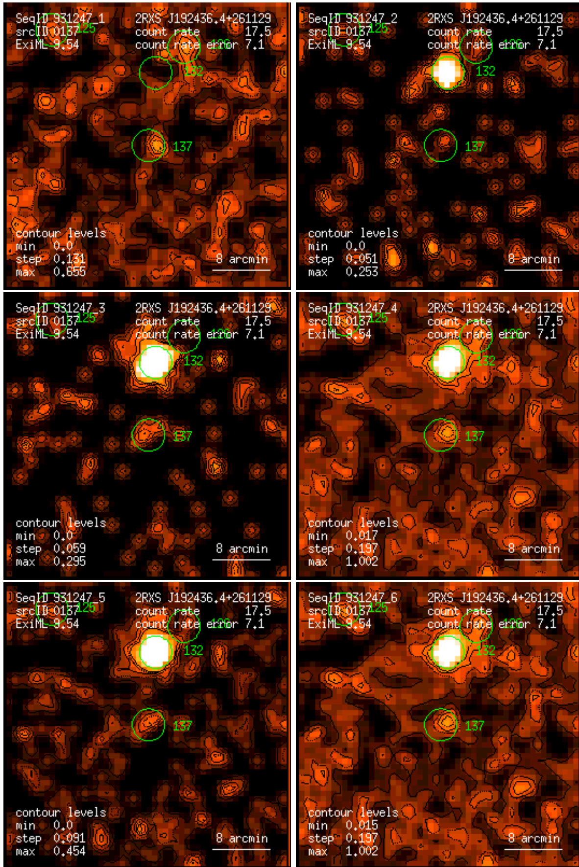
Figure 137: RASS 931247: detection 0137: band rate images, Gaussian filter: (1) PSPC channels 11 – 41, (2) 52 – 90, (3) 91 – 201, (4) 11 – 235, (5) 52 – 201, (6) 11 – 201. Broad band rates in counts/ks. Band rate contour levels in counts/ks/arcmin 2 .
