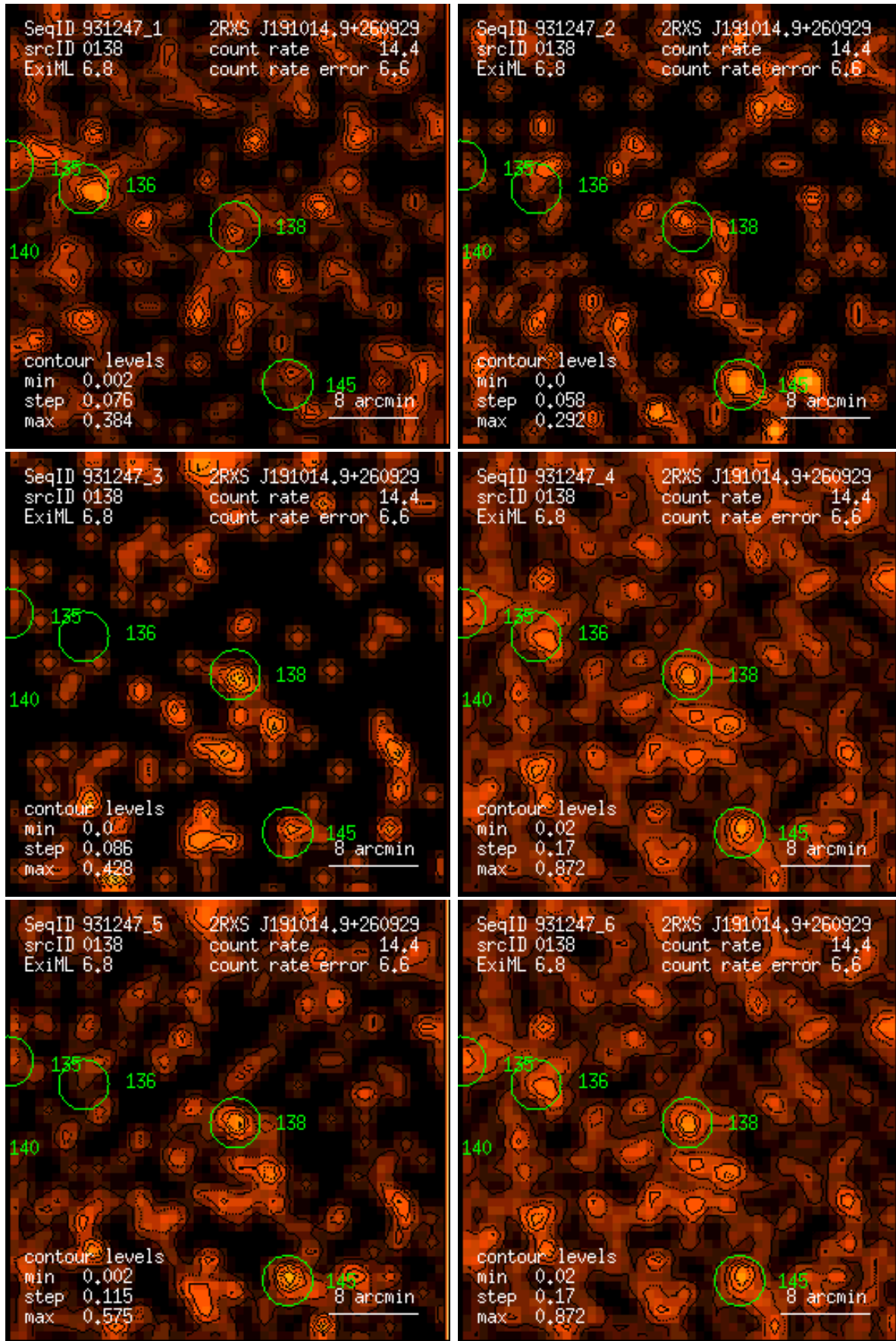
Figure 138: RASS 931247: detection 0138: band rate images, Gaussian filter: (1) PSPC channels 11 – 41, (2) 52 – 90, (3) 91 – 201, (4) 11 – 235, (5) 52 – 201, (6) 11 – 201. Broad band rates in counts/ks. Band rate contour levels in counts/ks/arcmin 2 .
