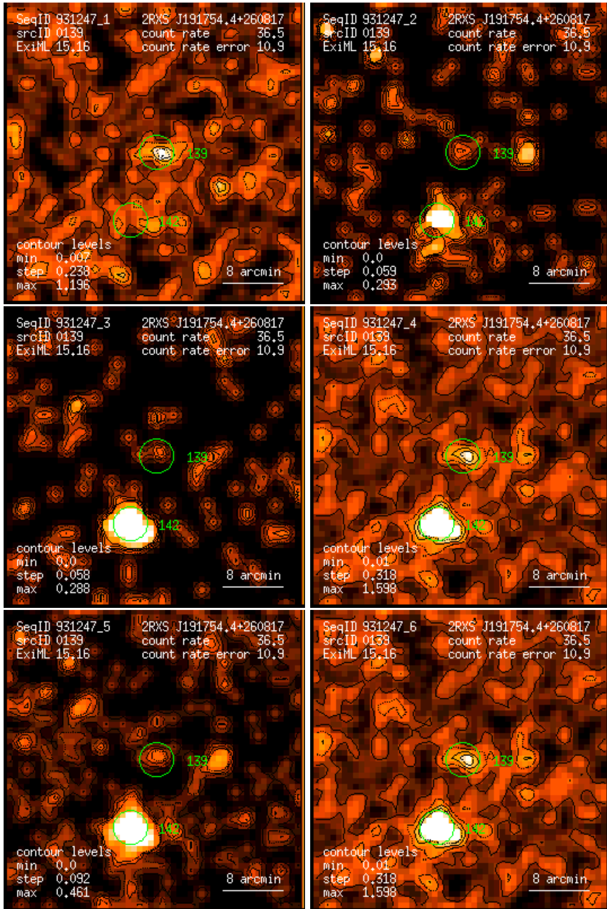
Figure 139: RASS 931247: detection 0139: band rate images, Gaussian filter: (1) PSPC channels 11 – 41, (2) 52 – 90, (3) 91 – 201, (4) 11 – 235, (5) 52 – 201, (6) 11 – 201. Broad band rates in counts/ks. Band rate contour levels in counts/ks/arcmin 2 .
