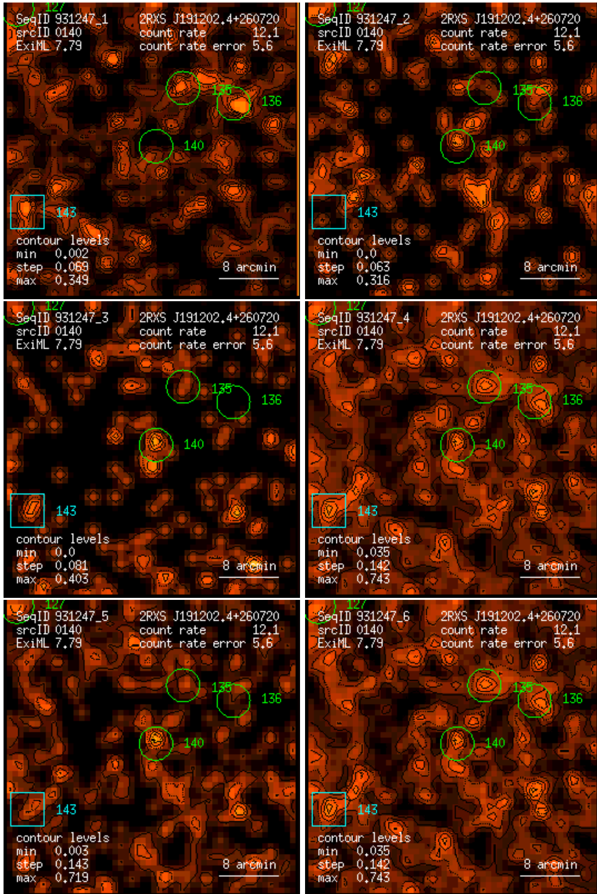
Figure 140: RASS 931247: detection 0140: band rate images, Gaussian filter: (1) PSPC channels 11 – 41, (2) 52 – 90, (3) 91 – 201, (4) 11 – 235, (5) 52 – 201, (6) 11 – 201. Broad band rates in counts/ks. Band rate contour levels in counts/ks/arcmin 2 .
