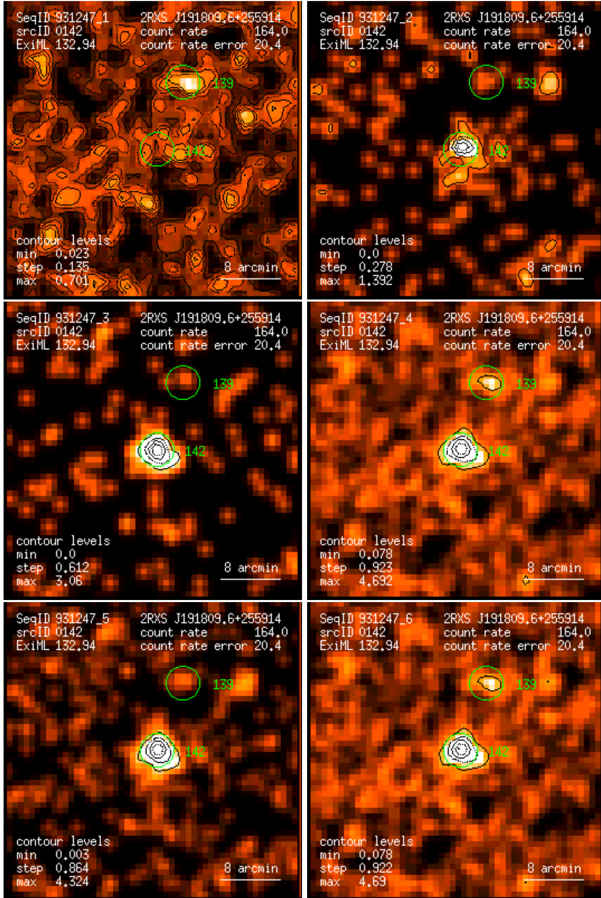
Figure 142: RASS 931247: detection 0142: band rate images, Gaussian filter: (1) PSPC channels 11 – 41, (2) 52 – 90, (3) 91 – 201, (4) 11 – 235, (5) 52 – 201, (6) 11 – 201. Broad band rates in counts/ks. Band rate contour levels in counts/ks/arcmin 2 .
