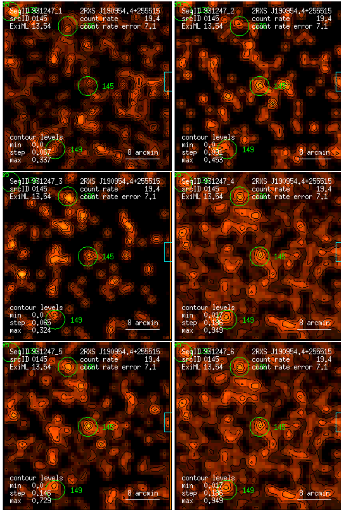
Figure 145: RASS 931247: detection 0145: band rate images, Gaussian filter: (1) PSPC channels 11 – 41, (2) 52 – 90, (3) 91 – 201, (4) 11 – 235, (5) 52 – 201, (6) 11 – 201. Broad band rates in counts/ks. Band rate contour levels in counts/ks/arcmin 2 .
