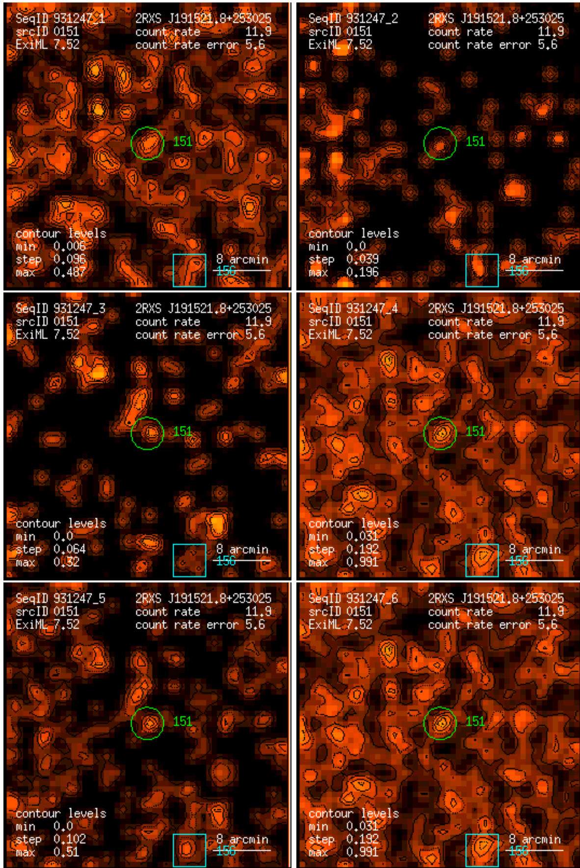
Figure 151: RASS 931247: detection 0151: band rate images, Gaussian filter: (1) PSPC channels 11 – 41, (2) 52 – 90, (3) 91 – 201, (4) 11 – 235, (5) 52 – 201, (6) 11 – 201. Broad band rates in counts/ks. Band rate contour levels in counts/ks/arcmin 2 .
