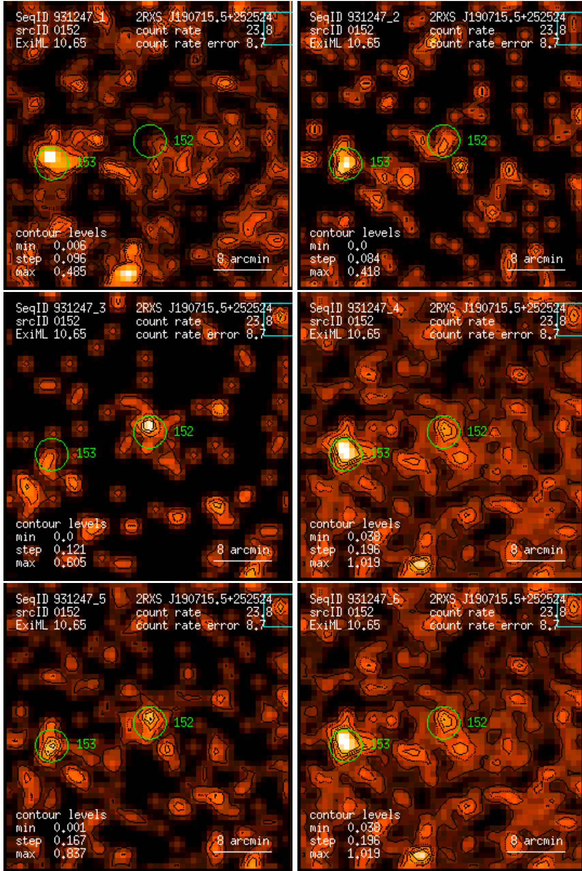
Figure 152: RASS 931247: detection 0152: band rate images, Gaussian filter: (1) PSPC channels 11 – 41, (2) 52 – 90, (3) 91 – 201, (4) 11 – 235, (5) 52 – 201, (6) 11 – 201. Broad band rates in counts/ks. Band rate contour levels in counts/ks/arcmin 2 .
