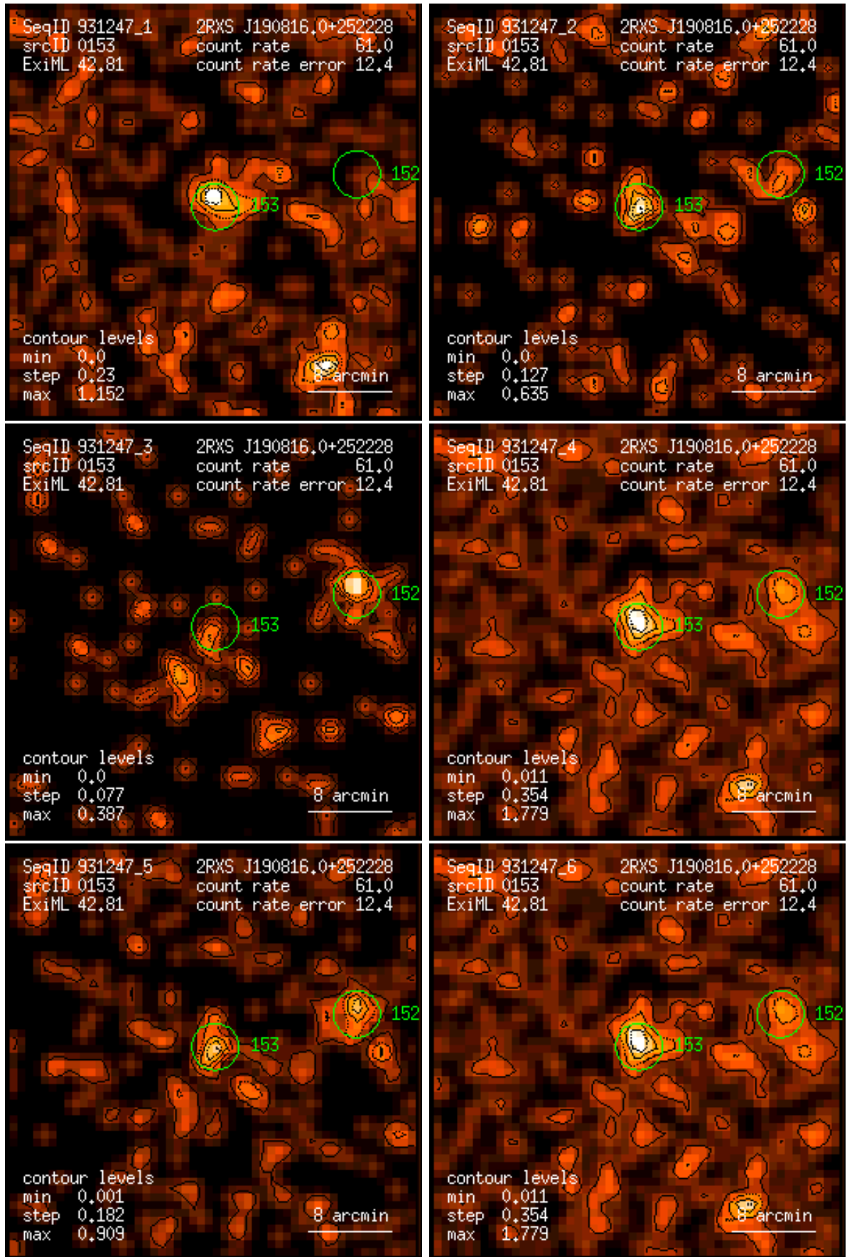
Figure 153: RASS 931247: detection 0153: band rate images, Gaussian filter: (1) PSPC channels 11 – 41, (2) 52 – 90, (3) 91 – 201, (4) 11 – 235, (5) 52 – 201, (6) 11 – 201. Broad band rates in counts/ks. Band rate contour levels in counts/ks/arcmin 2 .
