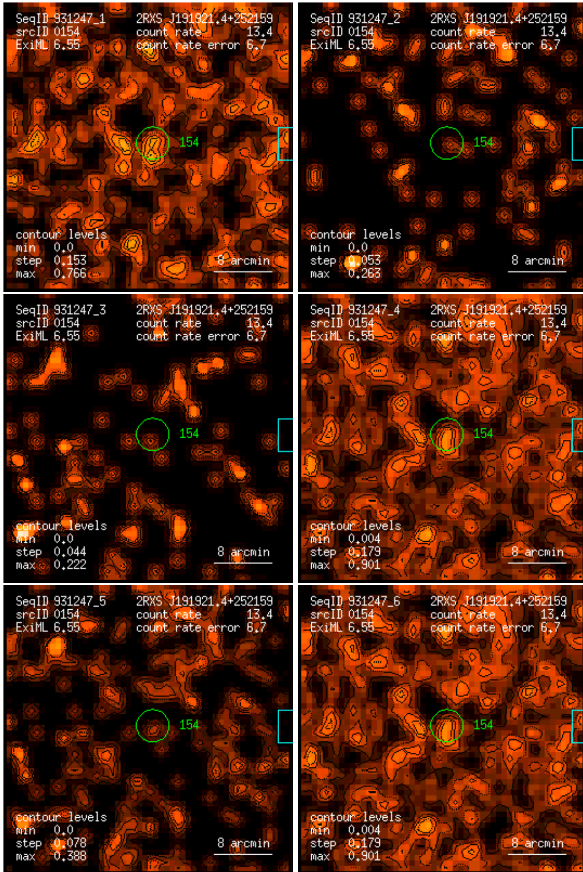
Figure 154: RASS 931247: detection 0154: band rate images, Gaussian filter: (1) PSPC channels 11 – 41, (2) 52 – 90, (3) 91 – 201, (4) 11 – 235, (5) 52 – 201, (6) 11 – 201. Broad band rates in counts/ks. Band rate contour levels in counts/ks/arcmin 2 .
