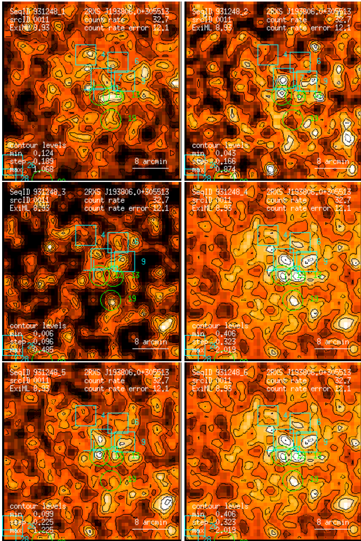
Figure 11: RASS 931248: detection 0011: band rate images, Gaussian filter: (1) PSPC channels 11 – 41, (2) 52 – 90, (3) 91 – 201, (4) 11 – 235, (5) 52 – 201, (6) 11 – 201. Broad band rates in counts/ks. Band rate contour levels in counts/ks/arcmin 2 .
