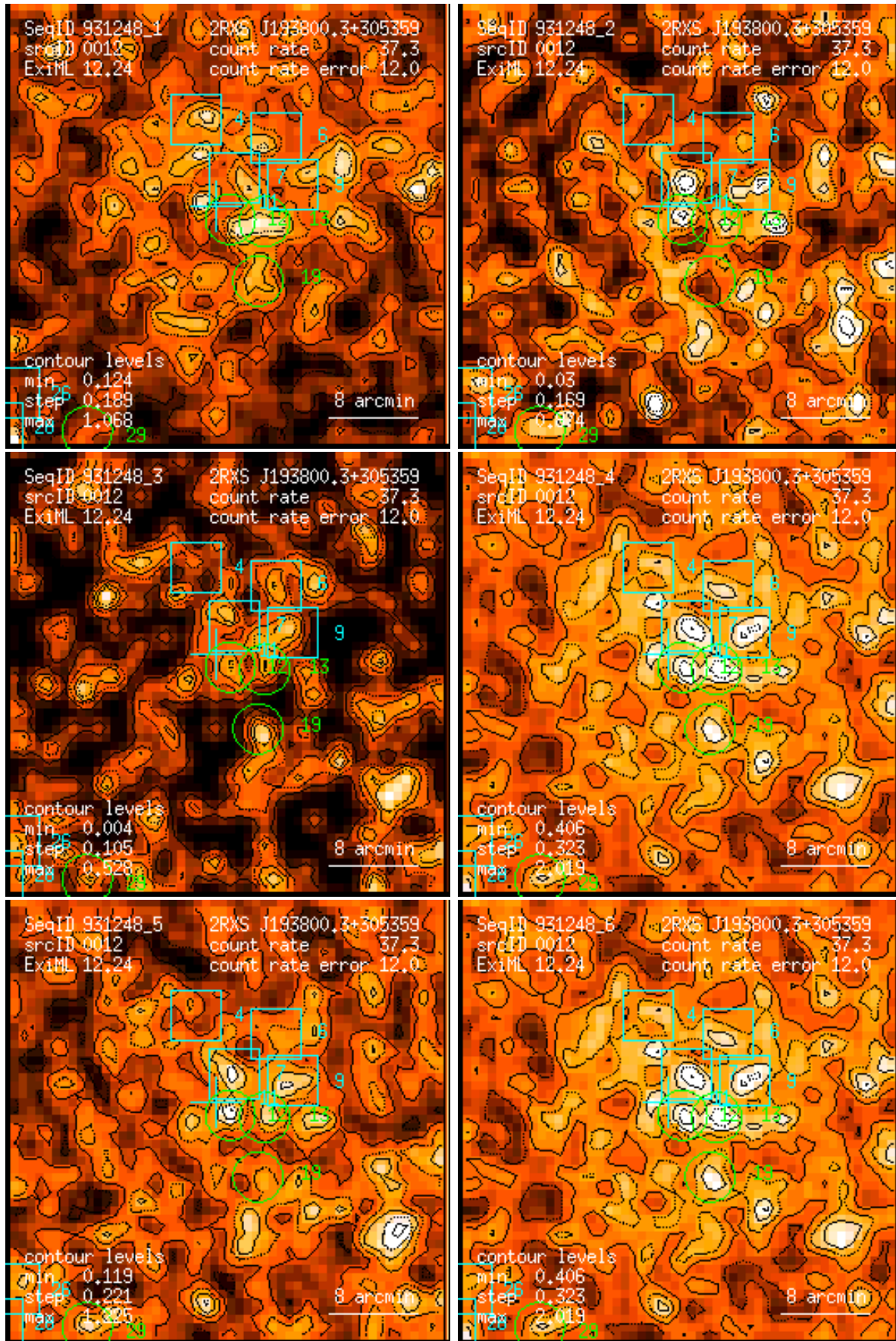
Figure 12: RASS 931248: detection 0012: band rate images, Gaussian filter: (1) PSPC channels 11 – 41, (2) 52 – 90, (3) 91 – 201, (4) 11 – 235, (5) 52 – 201, (6) 11 – 201. Broad band rates in counts/ks. Band rate contour levels in counts/ks/arcmin 2 .
