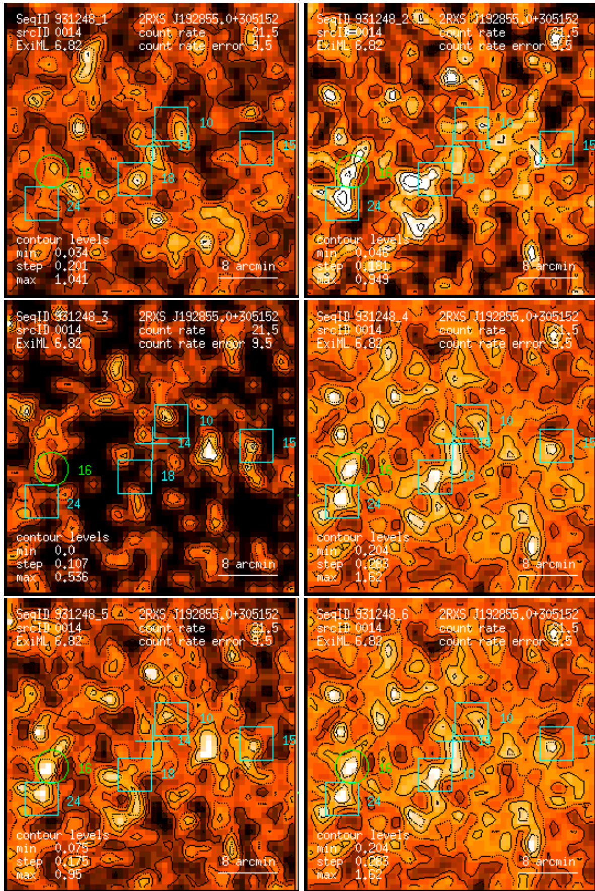
Figure 14: RASS 931248: detection 0014: band rate images, Gaussian filter: (1) PSPC channels 11 – 41, (2) 52 – 90, (3) 91 – 201, (4) 11 – 235, (5) 52 – 201, (6) 11 – 201. Broad band rates in counts/ks. Band rate contour levels in counts/ks/arcmin 2 .
