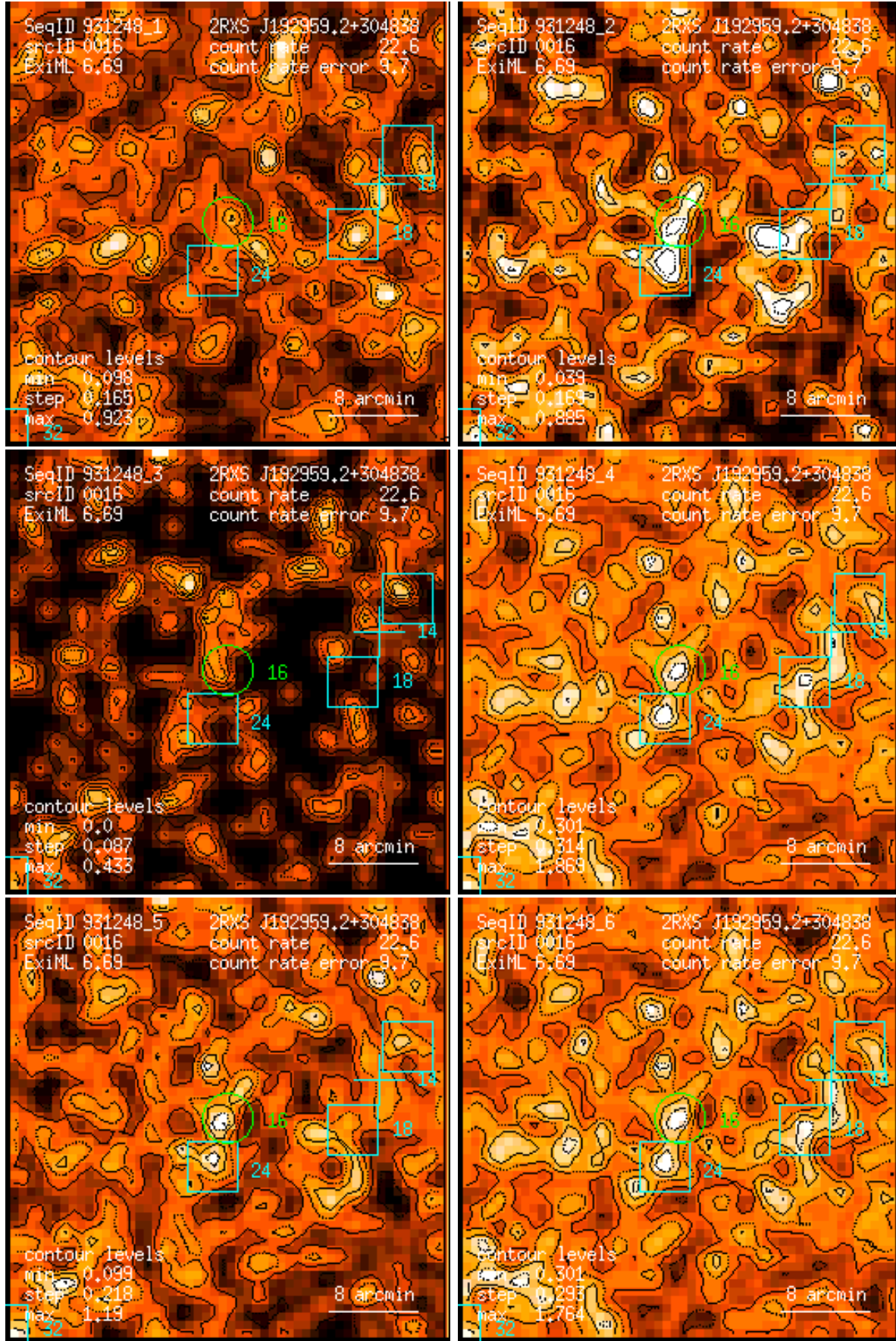
Figure 16: RASS 931248: detection 0016: band rate images, Gaussian filter: (1) PSPC channels 11 – 41, (2) 52 – 90, (3) 91 – 201, (4) 11 – 235, (5) 52 – 201, (6) 11 – 201. Broad band rates in counts/ks. Band rate contour levels in counts/ks/arcmin 2 .
